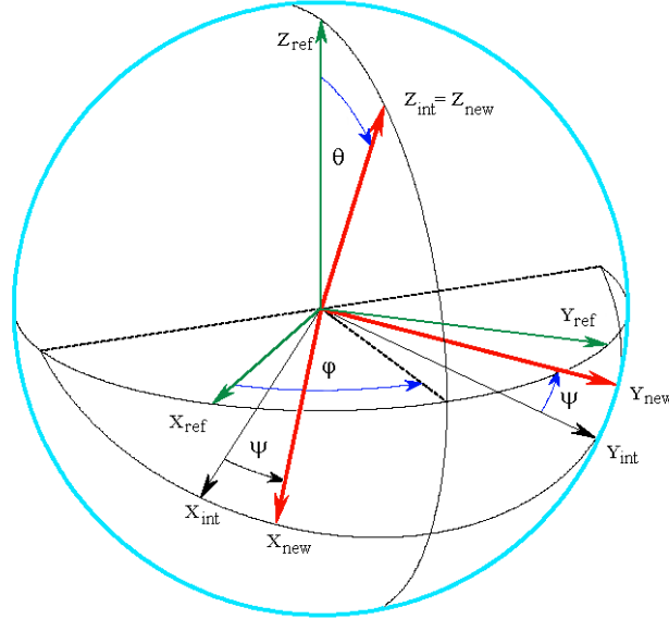
Figure 2: The orientation of the new coordinate system relative to the reference system specified by the angles \theta , \phi and \psi .
