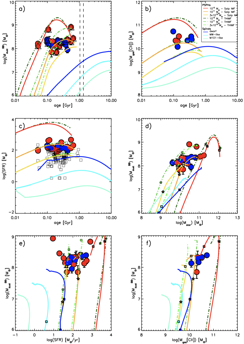
Fig. 2. Scaling relations of the ALPINE targets. Top panels: M_{\text{dust}} vs. age (panel a) and M_{\text{gas}} vs. age (b). Middle panels: SFR vs. age (c) and M_{\text{dust}} vs. M_{\text{star}} (d). Bottom panels: M_{\text{dust}} vs. SFR (e) and M_{\text{dust}} vs. M_{\text{gas}} (f). M_{\text{dust}} is computed by means of a MBB fit and assuming T = 25 K and \beta = 1.8 . The blue and red points show detections at 4 < z < 5 and 5 < z < 6 , respectively. In panel a the triangles around the points indicate galaxies classified as mergers or dispersion-dominated objects (Le Fèvre et al. 2020), whereas the black vertical dashed lines indicate the age of the Universe at redshift 4.5 and z = 5.5 (corresponding to an age of the Universe of 1.35 Gyr and 1.05 Gyr, respectively). The empty squares in panel c represent the ALPINE galaxies non-detected in continuum. The curves represent the chemical evolution models described in Sect. 4.1. The yellow, orange, and red solid lines represent proto-spheroid models of baryonic mass 3 \times 10^{10} , 10^{11} , and 10^{12} M_{\odot} , respectively, computed with a standard Salpeter IMF (Salpeter 1955). The light green, green, and dark green dot-dashed lines are for three PSPHs with the same baryonic masses as above, but characterised by a top-heavy IMF (Larson 1998). The light cyan, cyan, and blue solid lines represent models for a dwarf spiral, an intermediate-mass spiral, and an M101-like spiral, respectively (Calura et al. 2017). The stars and squares plotted along each curve and in the same colour indicate the evolutionary times of 0.1 and 0.5 Gyr, respectively.
