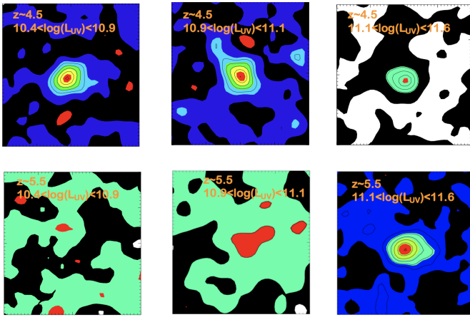
Fig. 3. 6'' \times 6'' cutouts of L_{\text{UV}} binned stacks of ALMA continuum images used to derive the stacked dust masses. The upper and lower panels show stacks of galaxies at z \sim 4.5 and z \sim 5.5 , respectively. The black solid contours show 2, 3, 4, 5\sigma . In the z \sim 4.5 bins all stacks have a clear detection at >4\sigma , but in the z \sim 5.5 bins the stacks have a clear detection only at the highest L_{\text{UV}} bin. In Table 1 the results of the stacking analysis are summarised, including the number of sources stacked in each bin of L_{\text{UV}} .
