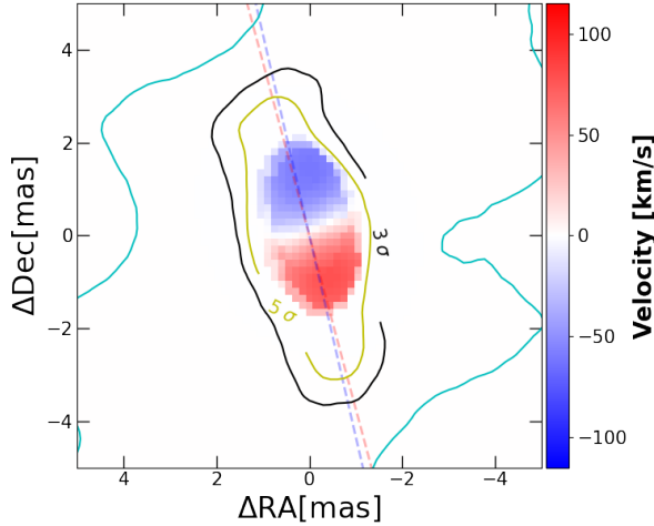
Fig. 5. Bry line first moment map (M1) obtained from the line velocity-dispersed images. For comparison, the 1, 3, and 5\sigma K -band continuum contours are overplotted in cyan, black, and yellow. The dashed red and blue lines illustrate the orientation of the semi-major axis of the continuum and the Bry line emission, respectively.
