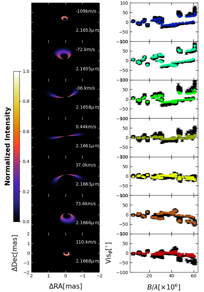
Fig. 6. Results of the Keplerian disk model fitting. Left: velocity maps from our Bry line Keplerian disk model. From top to bottom , we show velocity maps at: \sim -110 \text{ km s}^{-1} , \sim -73 \text{ km s}^{-1} , \sim -36 \text{ km s}^{-1} , \sim 0 \text{ km s}^{-1} , \sim 37 \text{ km s}^{-1} , \sim 74 \text{ km s}^{-1} , and \sim 110 \text{ km s}^{-1} . See the main text for details. Right: comparison between the observed continuum-corrected Bry line absolute phases (black dots) and those obtained from the Bry line Keplerian disk model shown in left panel (coloured dots).
