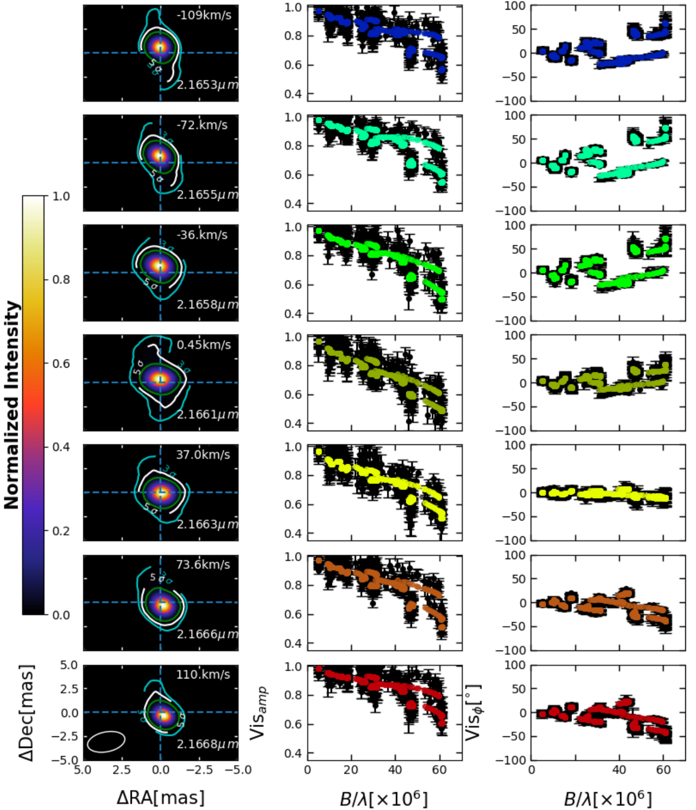
Fig. 4. Results of the image reconstruction. Left: H I Bry line reconstructed images of HD 58647. North is up, and east is to the left. Contours represent 3, 5, and 10 \sigma . Middle and right: comparison of the observed continuum-subtracted visibility amplitudes and absolute phases (black circles with error bars) with the synthetic observables extracted from the reconstructed image.
