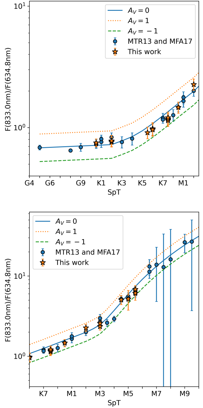
Fig. B.1. F_{\text{red}} = F(833\text{nm})/F(634.8\text{nm}) ratio calculated for the class III templates analyzed here (orange stars) as well as for the samples presented by MTR13 and MFA17 (blue circles). The error bars represent the uncertainties due to the noise in the spectra and do not include the uncertainty on the extinction correction. The blue line shows the value of F_{\text{red}} for A_V = 0 as a function of spectral type as derived by MFA17. The green and orange lines are obtained by dereddening and reddening the relationship of MFA17 by 1 mag respectively.
