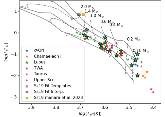
Fig. D.1. HRD containing the different results obtained for Sz19 for comparison the objects analyzed here (highlighted with larger black outlined markers) and those analyzed by MTR13 and MFA17 are displayed. The model isochrones and evolutionary tracks by Feiden (2016) are also shown. The isochrones are the 1.2, 3, 10 and 30 Myrs ones
