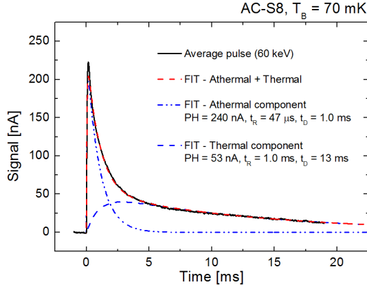
Fig. 3 Average 60 keV pulse acquired illuminating AC-S8 with a ^{241}\text{Am} source. The result of the double pulse fitting procedure is overplotted. (Color figure online)
