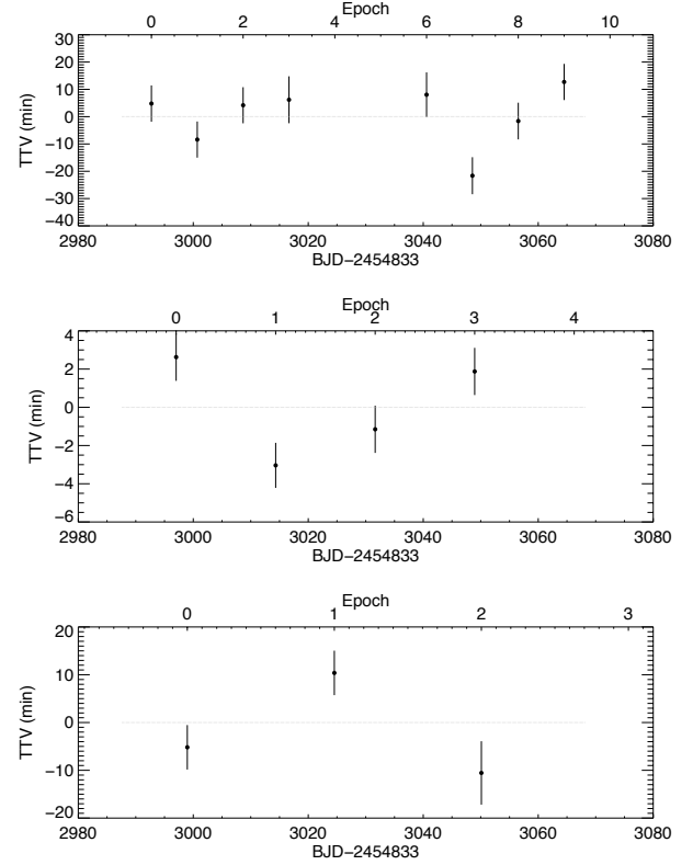
Figure 11. The individual transit times of the three planets. Transits that were severely affected by systematics were removed.
