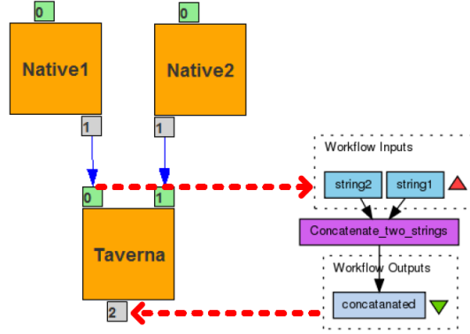
Figure 2: An example of meta-workflow. Two WS-PGRADE workflows modules (square box) are combined with a TAVERNA workflow module to concatenate two strings. Each module is actually a job to execute on the DCI. Each job communicates with other jobs within the workflow through job-owned input and output ports. An output port (small grey boxes) of a job connected with an input port (small green boxes) of a different job is called channel (blue arrow); these are directed edges of the graph. A single port must be either an input, or an output port of a given job.
