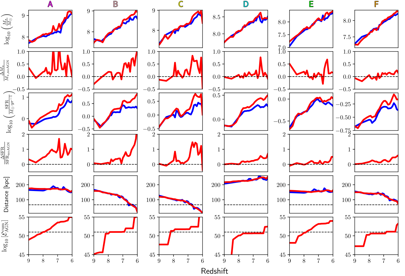
Figure 7. Redshift evolution of the six galaxies in the sample, as described in Section 4. From top to bottom: Stellar mass, stellar mass relative difference (i.e. [M_{*,\text{AGNcone}} - M_{*,\text{noAGN}}]/M_{*,\text{noAGN}} ), SFR, SFR relative difference (i.e. [\text{SFR}_{\text{AGNcone}} - \text{SFR}_{\text{noAGN}}]/\text{SFR}_{\text{noAGN}} ), distance from c_{\text{d}} , and \mathcal{E}_{\text{AGN}}^{\text{cum}} . The same colour coding of Fig. 3 is applied for the two runs. Horizontal lines mark the zero-level for the relative differences (second and forth rows), the time-averaged position of the cD virial radius (fifth row), and the threshold 10^{51} erg for the cumulative integrated flux (solid lines in sixth row; see Section 4.1).
