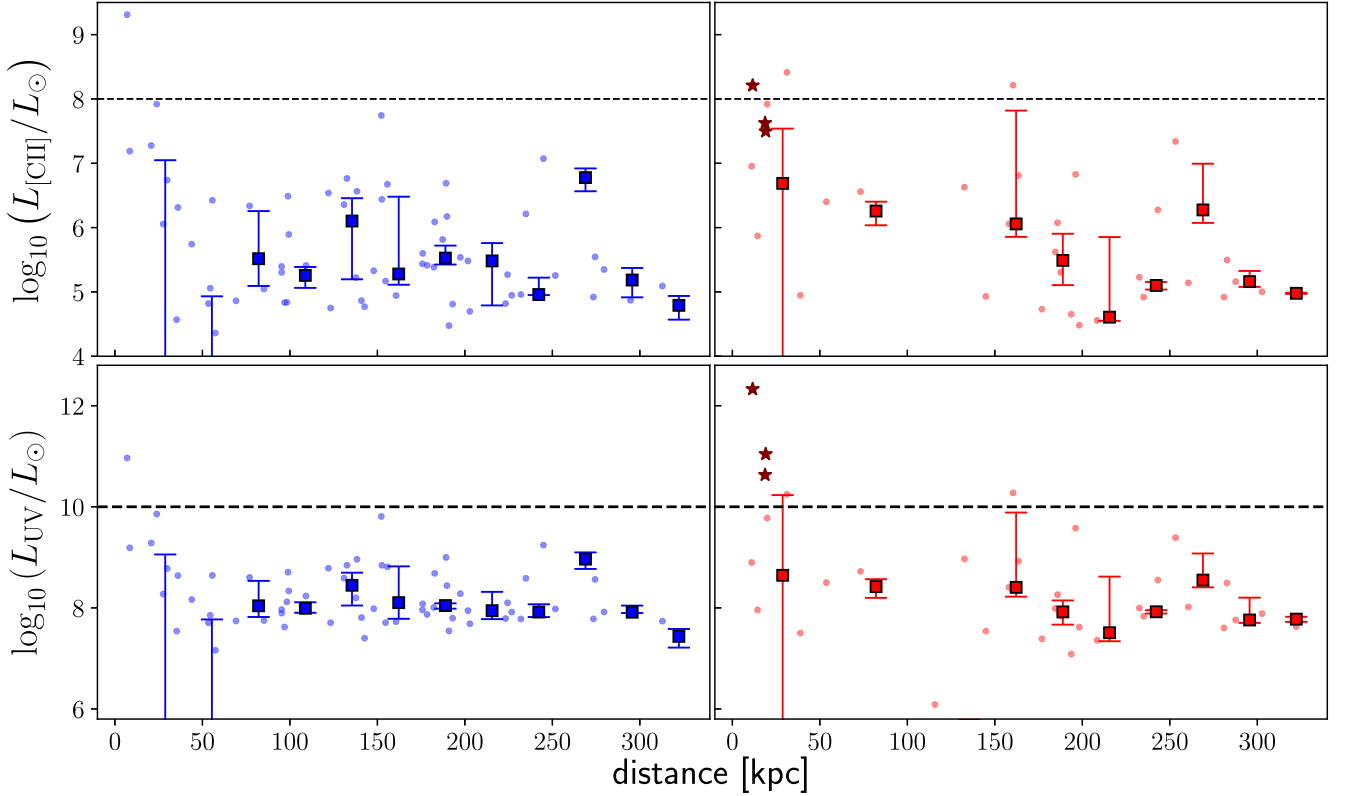
Figure 10. [C II] emission (top row) and UV emission (bottom row) as a function of distance from c_{\text{aw}} , for the same z = 6 sample of Fig. 5: noAGN on the left and AGNcone on the right . Horizontal dashed lines provide an estimate of the current instrumental sensitivities, derived from some of the deepest observations in the various bands. As in Fig. 5, where the brown stars mark the hosts of the most active AGN in AGNcone, the filled squares show the medians of the distributions and the error bars refer to the 30th and 70th percentiles. The values of the median points and the lower bounds of the error bars not shown in the plots are equal to zero.
