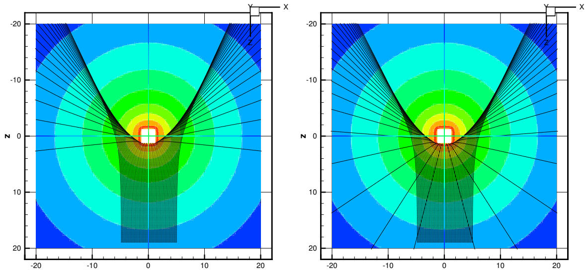
Fig. 10. Example of dust trajectories (particle size 0.1 \mu\text{m} , specific density 10^3 \text{ kg m}^{-3} , entrance velocity 93.0 \text{ m s}^{-1} ) in the electrostatic field of the Rosetta spacecraft. Left panel: case q/E_k = 0.230 \text{ C J}^{-1} (the particle charge is q = 4.172\text{e-}15 \text{ C} ). Right panel: case q/E_k = 0.246 \text{ C J}^{-1} (the particle charge is q = 4.450\text{e-}15 \text{ C} ).
