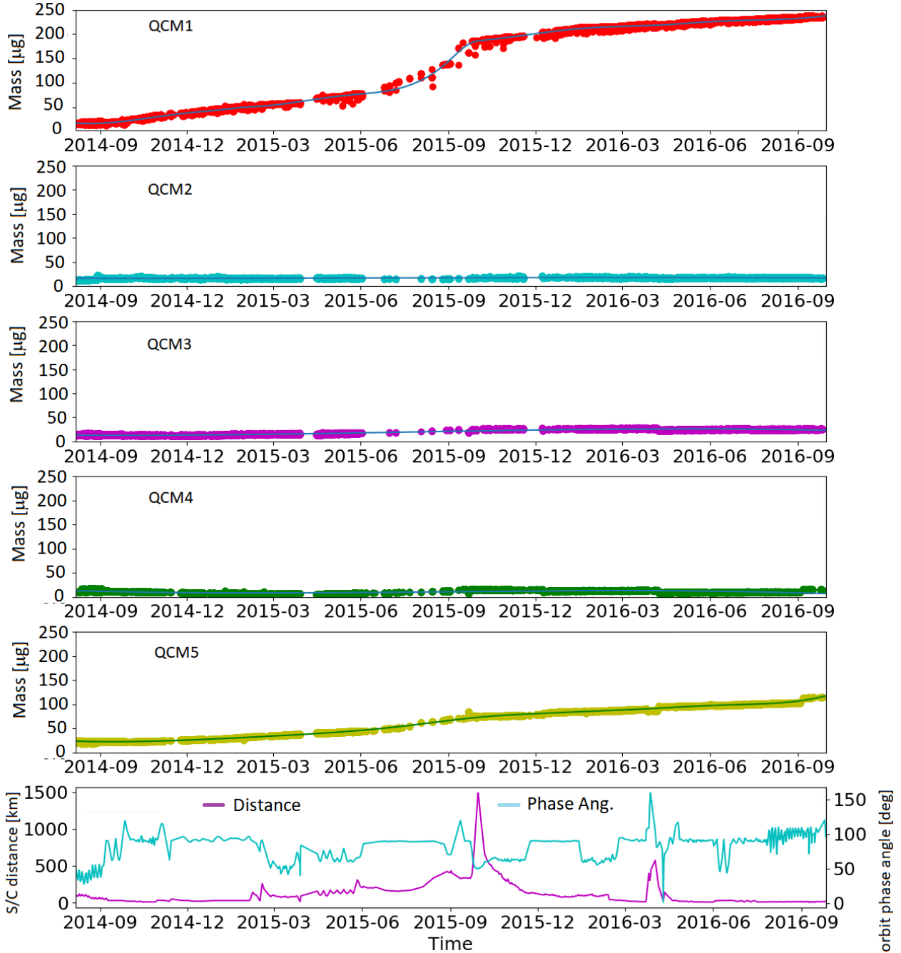
Fig. 4. Cumulated mass deposited on the QCMs retrieved after the isotherm filtering, i.e., on selected data points that were acquired when the QCM is at its most frequent temperature \pm 0.75^\circ\text{C} . Cumulated masses are fitted by continuous spline curves. The curves show a relevant mass deposition increase on QCM1 and QCM5, in particular around perihelion of 67P (13 August 2015). No dust mass increase is detected by QCM2 and QCM4, while a slight increase in QCM3 is limited to perihelion. In the bottom panel we report the variation of the S/C distance from the comet and the phase angle (spacecraft-comet-Sun) that could influence the dust flux. No clear correlation is visible. A dust flux increase is visible for QCM5 at the end of the mission, which is associated with the outburst that occurred on 5 September 2016, when the S/C was at about 5 km from the nucleus surface of 67P.
