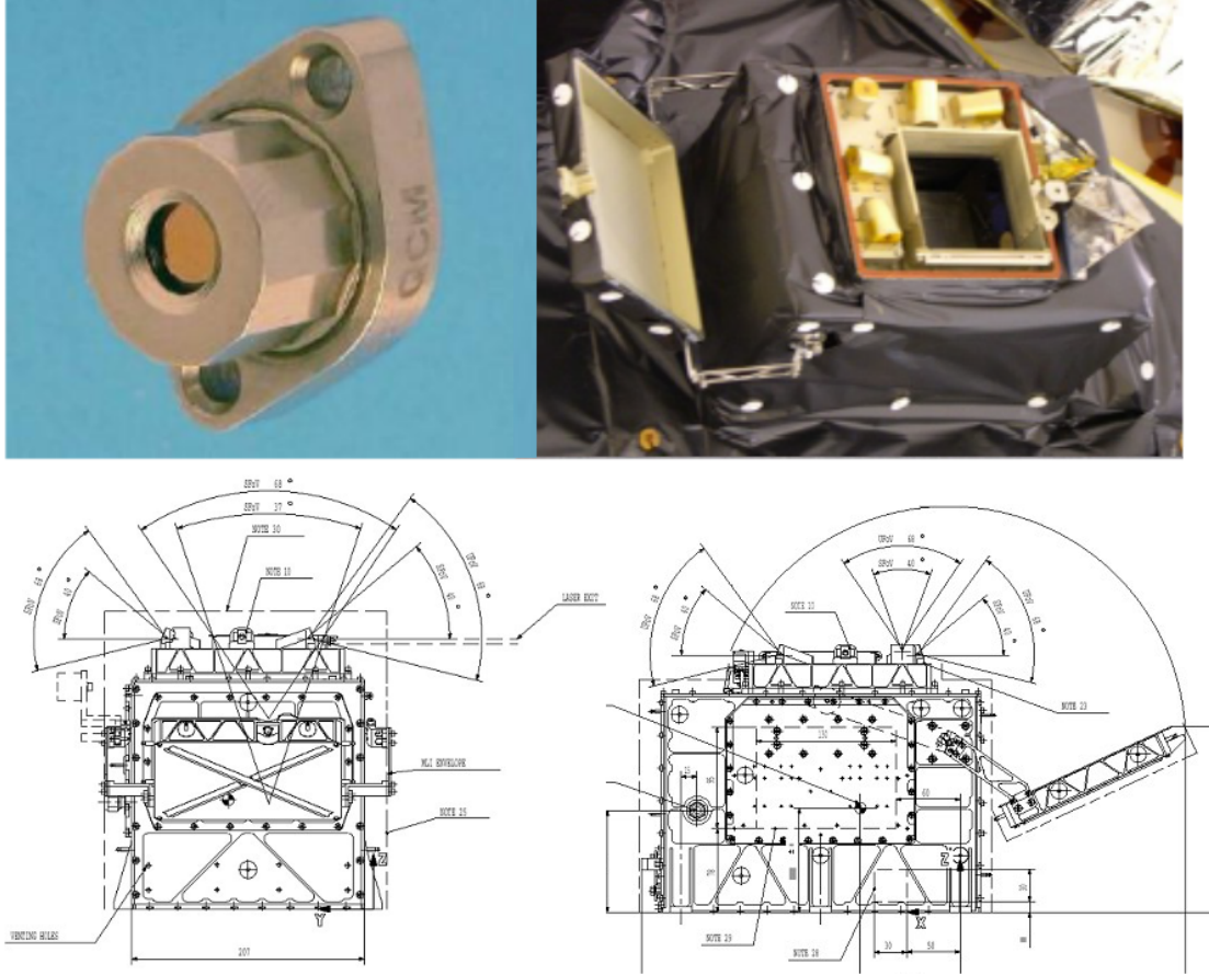
Fig. 1. MBS subsystem: one QCM-Research-MK21 sensor ( top left ); MBS subsystem mounted on GIADA integrated on board Rosetta ( top right ). Mechanical MBS configuration on GIADA. The QCMs FOV, 40° ( bottom left ), and the unobstructed FOV, 68° ( bottom right ) are highlighted.
