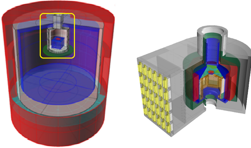
Fig. 6: Left - The cryostat mass model used in older Geant4 simulations. The FPA model is inside the yellow box. Right - The updated FPA mass model. It can be seen the much higher degree of complexity with respect to the previous one.
