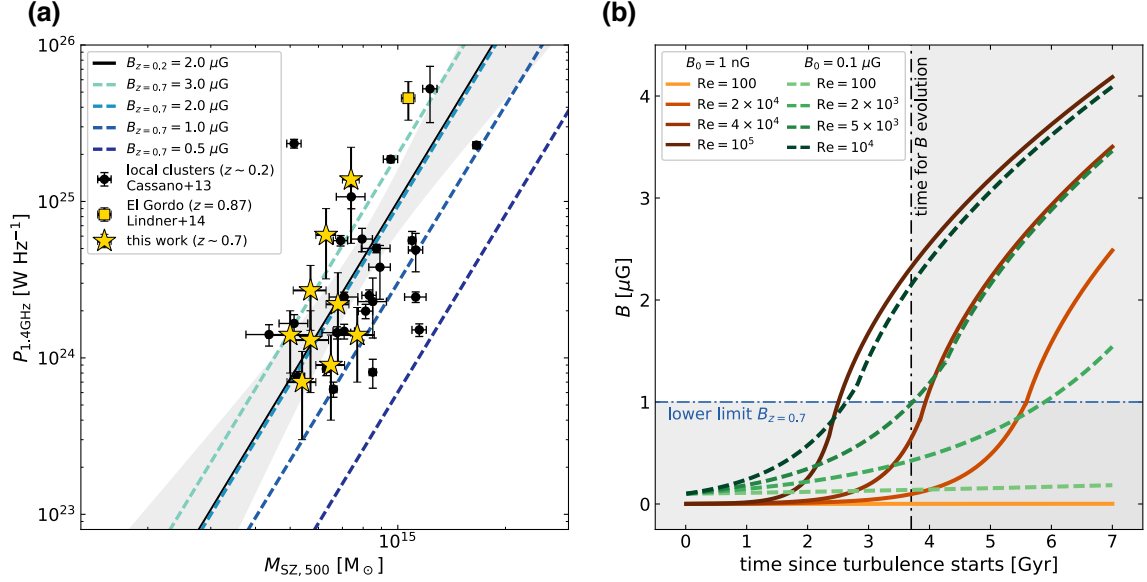
Figure 3: Cluster magnetic field estimation and theoretical magnetic field evolution. Panel (a): P_{1.4\text{GHz}}-M_{500} diagram for nearby ( \text{median}(z) \sim 0.2 , black dots [15]) and distant ( \text{median}(z) \sim 0.7 , yellow stars) radio halos, including that in El Gordo ( z = 0.87 [20], yellow square). Error bars on the yellow stars are obtained with 100 Monte Carlo realization of the radio luminosity, including flux density and spectral index uncertainties, while error bars on the black dots and yellow square are given by the literature. The black solid line represents the best-fit relation from the low-redshift sample, with the 95% level confidence (grey area). The blue dashed lines represent, from light to darker colors, the theoretical relations at high- z taking magnetic field strengths of 3.0, 2.0, 1.0 and 0.5 \mu\text{G} (assuming a typical local cluster magnetic field of 2 \mu\text{G} ). Panel (b): Magnetic field growth since the start of the turbulence, based on the small-scale dynamo theory. The initial fields, B_0 , are set at 1 nG (solid orange lines; from light to darker colors: \text{Re} = [100, 2 \times 10^4, 4 \times 10^4, 10^5] ) and 0.1 \mu\text{G} (dashed green lines; from light to darker colors: \text{Re} = [100, 2 \times 10^3, 5 \times 10^3, 10^4] ). The horizontal blue dot-dashed line sets the lower limit of the magnetic field strength in distant galaxy clusters (see panel (a)). The vertical black dot-dashed line shows the upper limit on the approximate time available for the magnetic field growth (see Methods).
