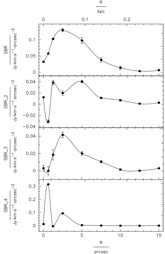
Fig. 15. Final parametrization: surface brightness. Negative values might reflect statistical errors, but might also be due to absorption. From top to bottom we present c- \text{C}_3\text{H}_2 J = 2_{12} \rightarrow 1_{10} (SBR), \text{CH}_3\text{C}_2\text{H} 5_0 \rightarrow 4_0 (SBR-2) and, overlapping, c- \text{C}_3\text{H}_2 J = 4_{32} \rightarrow 4_{23} (SBR-3) and \text{H}42\alpha (SBR-4; see Table 1 for details to the transitions). The abscissa shows galactocentric radii and the ordinate shows emission in units of \text{Jy km s}^{-1} \text{arcsec}^{-2} . Further information is given in Sect. 4.6.2.
