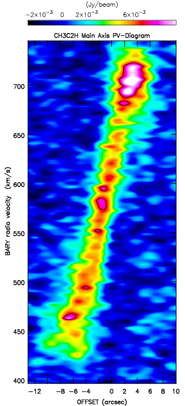
Fig. 14. Position-velocity plot of \text{CH}_3\text{C}_2\text{H } 5_0 \rightarrow 4_0 along the major axis with the abscissa scaled relative to the continuum peak. Contour: 7 \text{ mJy beam}^{-1} . The plot emphasizes (1) the clumpiness of the gas, (2) the steepening of the rotation curve between barycentric V \approx 500 \text{ km s}^{-1} and the systemic velocity of V \approx 571 \text{ km s}^{-1} and (3) its flattening between 470 and 500 \text{ km s}^{-1} .
