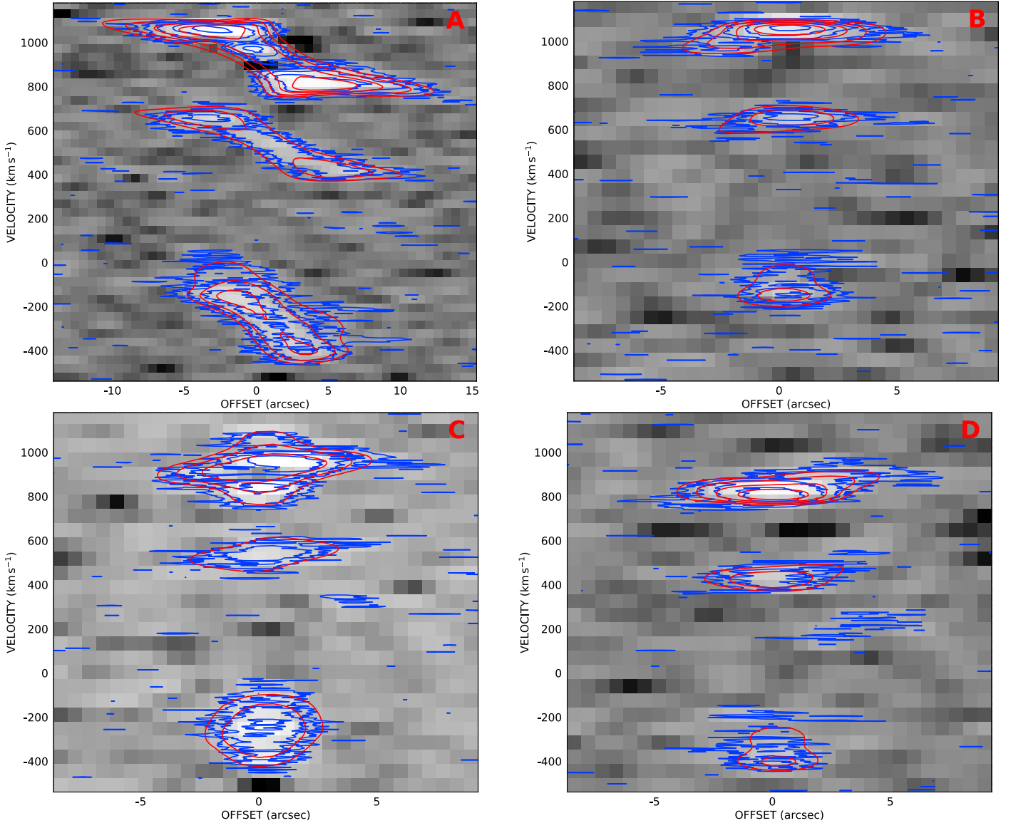
Fig. 20. PV-diagrams along the lines shown in Fig. 19, each with (from top to bottom) \text{c-C}_3\text{H}_2 2_{12} \rightarrow 1_{01} , \text{CH}_3\text{C}_2\text{H} 5_0 \rightarrow 4_0 and, overlapping, \text{C}_3\text{H}_2 4_{32} \rightarrow 4_{23} and \text{H}42\alpha . The velocity scale refers to that of the \text{CH}_3\text{C}_2\text{H} line (see Sect. 4.6.2 and Table 1). Dark: low intensity; light gray: high intensity. Top left panel: cut A (see also Fig. 19) along the major axis from the northeast toward the southwest. Top right panel: cut B perpendicular to the major axis crossing the 710 \text{ km s}^{-1} peak from the southeast toward the northwest. Bottom left panel: cut C perpendicular to the major axis, central line. Bottom right panel: cut D perpendicular to the major axis crossing the 430 \text{ km s}^{-1} peak. A, B, C or D are displayed in the upper right corner of their respective panels. Blue contours: original data cube. Red contours: model data cube with constant vertical gradient in radial motion and final rotation curve (see top two panels of Fig. 16). Contours: 0.1, 0.2, 0.4, 0.8 \text{ mJy beam}^{-1} .
