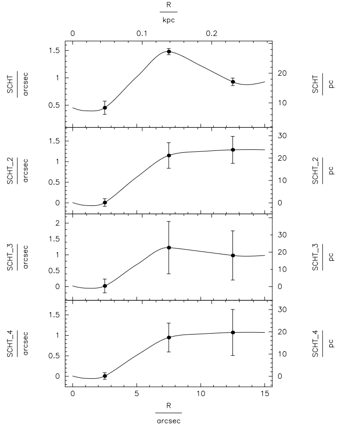
Fig. 17. Final parametrization: full scale height. From top to bottom: in the same order as in Fig. 15, \text{c-C}_3\text{H}_2 (SCHT), \text{CH}_3\text{C}_2\text{H} (SCHT-2) and, overlapping, \text{c-C}_3\text{H}_2 (SCHT-3) and \text{H}42\alpha (SCHT-4). The ordinate on the left-hand side shows scale height in arcseconds; the ordinate on the right-hand side denotes scale height in pc, both as a function of galactocentric radius.
