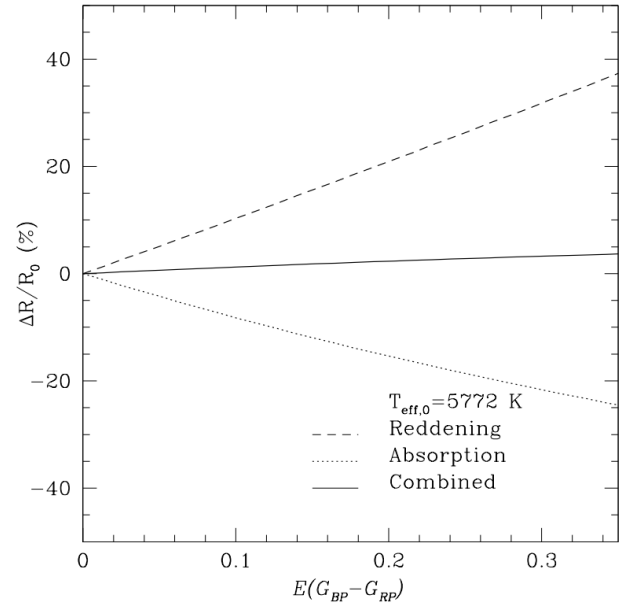
Fig. F.1. Percentage variation of the apparent radius R estimated neglecting the presence both of absorption and reddening, with respect to the true radius R_0 of a solar-type star (with effective temperature T_{\text{eff}}=5772 K) as a function of reddening E(G_{BP} - G_{RP}) (solid line). The dashed and dotted lines represent the apparent radius variation resulting from neglecting either the reddening (dashed) or the absorption (dotted), respectively.
