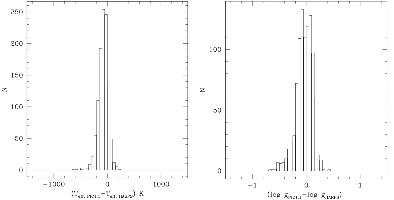
Fig. 18. Distributions of effective temperatures, and stellar gravity differences between asPIC1.1 and the HARPS sample.
