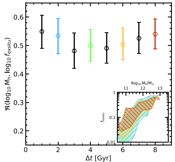
Figure C1. Correlation coefficient for different time intervals with 1 \sigma uncertainties indicated by error bars. The inset plot shows a region enclosing the 1 \sigma scatter for the M_h - f_{\text{exsitu}} relation for \Delta t = [2, 4, 6, 8] where the colour of the region corresponds to the value \Delta t indicated by the coloured error bars in the main plot.
