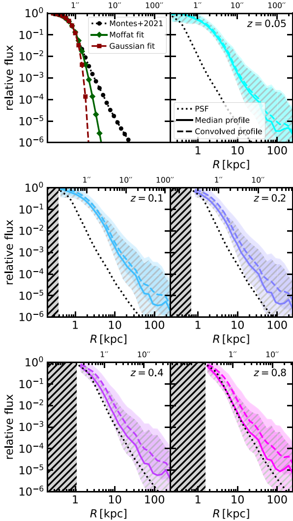
Figure B1. Top left-hand panel: Comparison of the measured 1D PSF from Montes et al. (2021) with a the best fit Moffat (1969) and Gaussian distributions. Other panels: surface brightness profiles compared to the PSF for different redshifts (indicated in the top right-hand corner of each panel). The solid lines show the median relative surface brightness profile of the raw mock images, dashed lines show the median relative surface brightness profiles after they have been convolved with the PSF, and the dotted black line shows the Montes et al. (2021) PSF. Coloured filled regions indicate the central 68th percentile (1 \sigma ) of profiles where the hatched region indicates the unconvolved profile. The x-axis limits are fixed in physical units between 0.2 and 250 kpc with the equivalent scale in arcseconds for each redshift shown on the top x-axis of each panel. The grey hatched region indicates radii smaller than the 0.2 arcsec Rubin Observatory pixel size.
