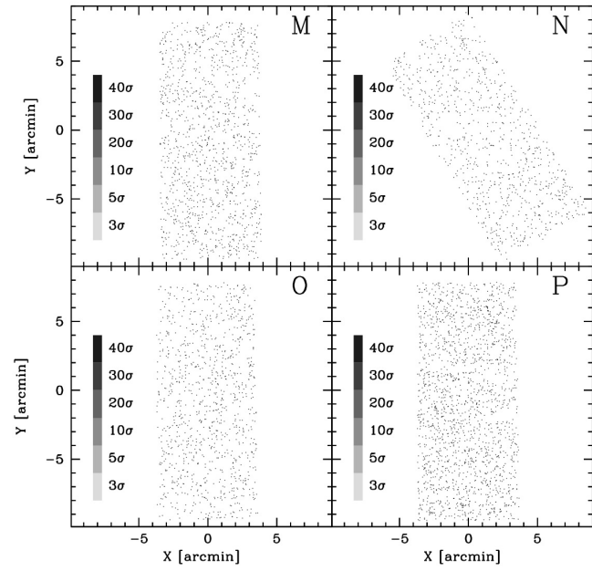
Fig. C.3. r27 maps and r25 maps fields M, N, O, and P. The arrangement and the meaning of the symbols are the same as in Fig. 9.
