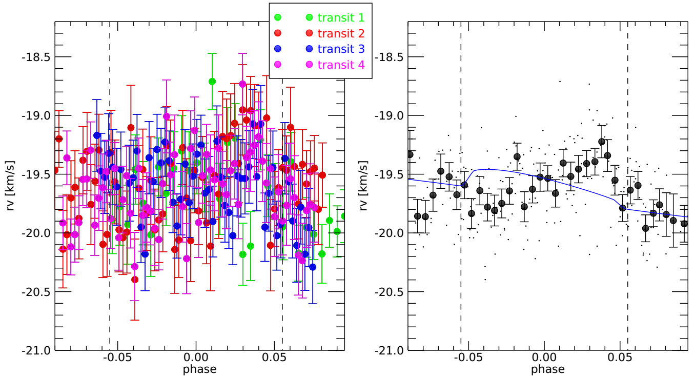
Fig. 4. (Left panel) Phase-folded RVs of the four HARPS-N transits of KELT-9b. Different colours refer to different transits. (Right panel) Mean RVs of the four transits (filled circles), together with single RVs (small dots). The theoretical RV solution (blue line) computed using Keplerian motion and the classical RML effect alone clearly does not match the observations. The vertical dashed lines show the ingress and egress of transit.
