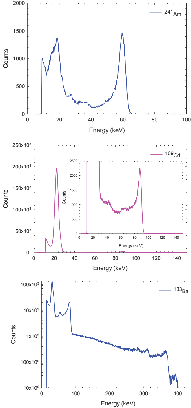
Fig. 5. Energy spectra recorded at different energies of the incident photons, by irradiating the detector with ^{241}\text{Am} (top), ^{109}\text{Cd} (center) and ^{133}\text{Ba} (bottom).
