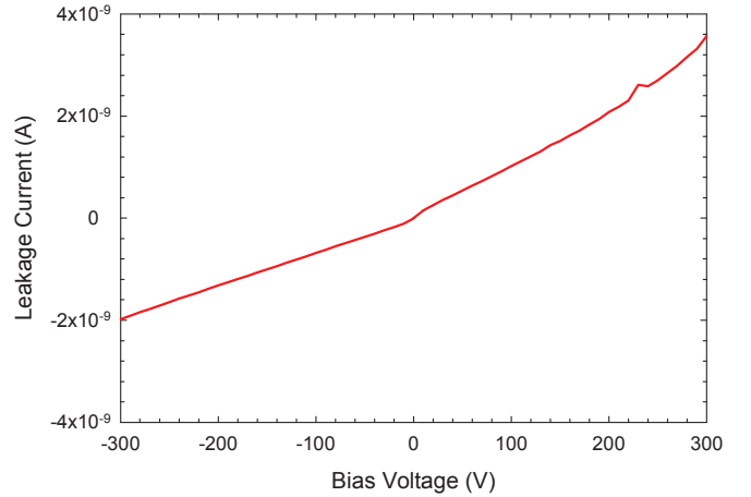
Fig. 3. Leakage current vs. bias voltage.
