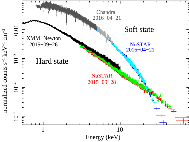
Figure 1. XMM-Newton , NuSTAR and Chandra spectra of MXB 1659-298 during the 2015-2017 outburst. Both the XMM-Newton (black) and the NuSTAR (red and green) spectra accumulated on 2015-09-26 and 2015-09-28, respectively, show a hard power law shape characteristic of the hard state. The simultaneous Chandra (light and dark grey) and the NuSTAR (light and dark blue) spectra obtained in 2016-04-21 show a significantly softer and brighter emission below \sim 20 keV, with a significant drop above \sim 20 - 30 keV.
