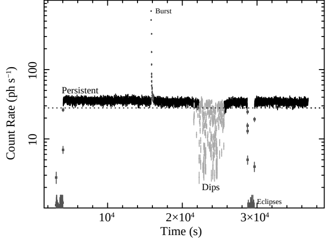
Figure 8. 0.5-10 keV XMM-Newton light curve of MXB 1659-298 performed on 2015-09-26. The EPIC-pn exposure starts just before the eclipsed period (shown with dark grey squares). During the observation a clear burst is observed (shown with dark grey colours) as well as intense dipping activity (light grey colours). The black points show the persistent emission. The dotted line indicates the lower bound we use to identify persistent flux, with intervals dipping below this being selected as dips. Time bins of 10 s are used.
