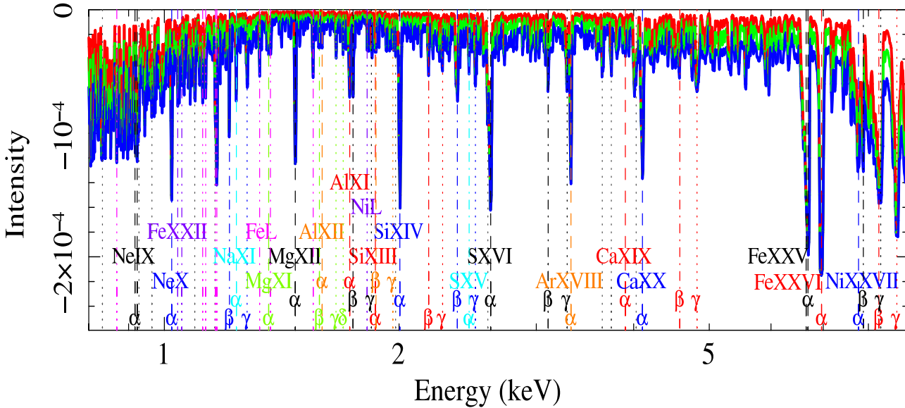
Figure 4. Residuals to the presence of narrow ( \sigma = 1 \text{ eV} ) absorption lines in the Chandra HETG (HEG+MEG) spectra. The red, green and blue solid lines show the 68, 90 and 99 % confidence contours. Sixty absorption lines are detected. We highlight with a vertical line each detected absorption feature. The same colour is used for features associated to the same series. In particular, the energies of the \alpha , \beta and \gamma transitions are reported with dashed, dash-dotted and dotted lines, respectively. Absorption lines associated with Fe L features are highlighted with magenta dot-dot-dot-dashed lines (in violet is the density sensitive Fe XXII doublet). Unidentified lines are shown with grey dotted lines.
