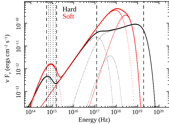
Figure 3. In black and red are shown the de-absorbed best fit "bona fide" spectral energy distribution during the hard and soft state, respectively. The dashed lines show the extremes of the X-ray and optical-UV energy ranges constrained by NuSTAR , XMM-Newton , Chandra and the Swift filters. The dotted vertical lines show the mean energy of the various filters.
