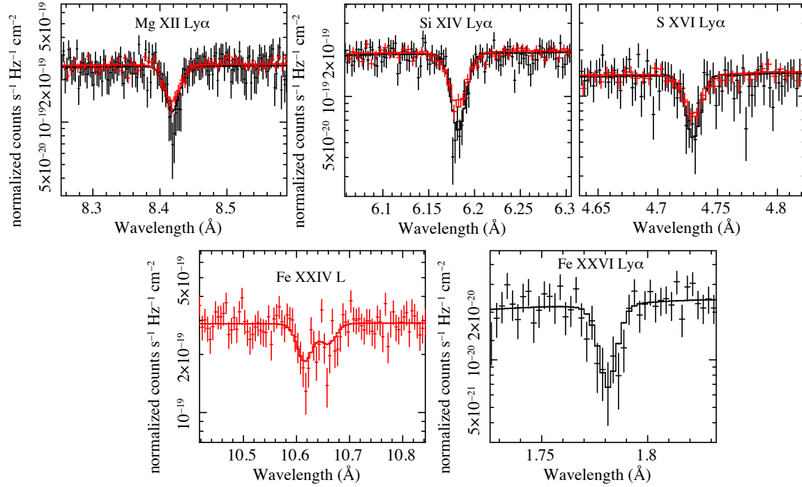
Figure 5. The red and black data display the Chandra HETG MEG and HEG spectra at the energies of some of the strongest lines, respectively, fitted with the best fit model (B7 in Tab. 1). ( Top panels ) from left to right show the Mg XII Ly \alpha , Si XIV Ly \alpha and S XVI Ly \alpha lines. The profile of all lines is well reproduced by the best fit photo-ionised absorption component. ( Bottom panels ) from left to right show the two lines of the Fe XXIV L complex and the Fe XXVI Ly \alpha transition. Only data of the MEG and HEG instruments are shown because of their higher effective area at low and high energies, respectively.
