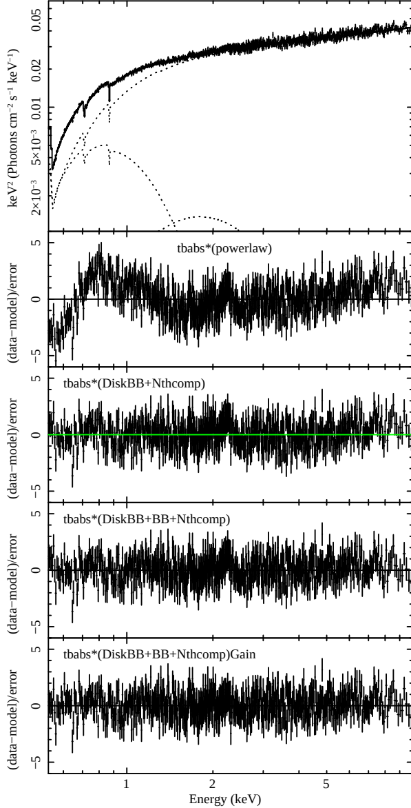
Figure 9. (Top panel) XMM-Newton EPIC-pn hard state spectrum fitted by the best fit model (disc black body plus blackbody and a dominant Comptonisation components absorbed by neutral material). No signs of ionised absorption is present. (Centre top panel) Residuals once the data are fitted with an absorbed power law. (Centre panel) Residuals after fitting with an absorbed disk black body plus Comptonisation model. (Centre bottom panel) Residuals after the addition of a black body component. (Bottom panel) Residuals after the consideration of a gain offset in the response files.
