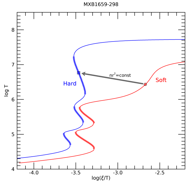
Figure 7. Photoionisation stability curves of the ionised absorbing plasma when illuminated with the soft (red) and hard (blue) SEDs. The thick segments indicate the thermally unstable branches of the curves. The red circle indicates the position of the ionised absorber during the soft state. The absorber is thermally stable. The blue square indicates the expected condition of the absorber when illuminated by the hard state SED. Such conditions are thermally unstable.
