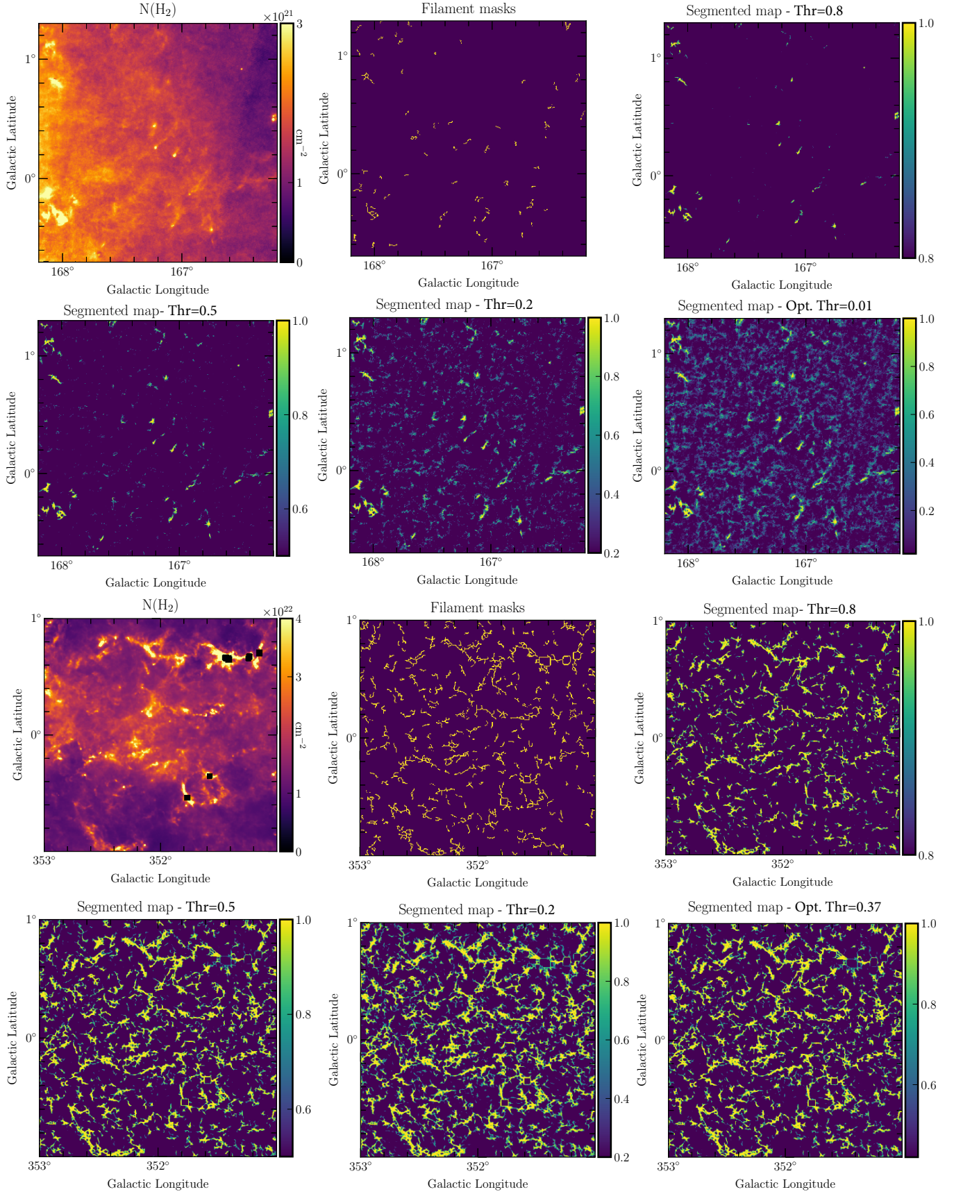
Fig. 18. Zoom-in on the evolution of segmentation results as a function of the classification threshold showing the filamentary structures estimated by UNet++ 10^{-3} in 160\text{--}171^\circ (six top images) and 349\text{--}356^\circ (six bottom images) regions of the Galactic plane. The original \text{H}_2 column density image (top left in each group), the ground-truth input filament mask, and the corresponding segmented image at different thresholds (0.8, 0.5, 0.2, and the optimal threshold) are shown from top left to bottom right. The regions are 2^\circ \times 2^\circ wide.
