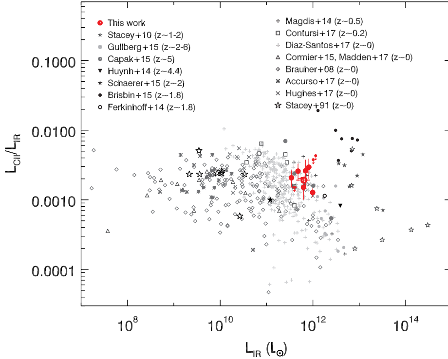
Figure 6. Ratio between the [C II] and IR (8 – 1000 \mu\text{m} ) luminosity of our sample galaxies, as a function of the IR luminosity. Different symbols indicate distinct datasets: our [C II] detections (large red filled circles), our [C II] upper limits for the non-detections (small red filled circles), the average value of our sample (empty red circle), Stacey et al. (2010, grey filled stars indicate star-forming galaxies, grey empty stars indicate AGN or starbursts), Stacey et al. (1991, black empty stars), Gullberg et al. (2015, light grey filled circles), Capak et al. (2015, dark grey filled circles indicate their measurements, dark grey empty circles indicate the stack of their non detections), Diaz-Santos et al. (2017, grey crosses), Cormier et al. (2015, black triangles), Brauher et al. (2008, grey diamond), Contursi et al. (2017, grey squares), Magdis et al. (2014, dark grey crosses), Huynh et al. (2014, black downward triangle), Schaefer et al. (2015, black filled star), Brisbin et al. (2015, black filled circles), Ferkinhoff et al. (2014, black empty circle), Hughes et al. (2017, grey crosses), Accurso et al. (2017a, grey asterisks). We note that we are plotting the de-magnified IR luminosity for the sample of lensed galaxies by Gullberg et al. (2015): we considered that the [C II] emission line is magnified by the same factor as the IR (see discussion in the text and Gullberg et al. 2015). The magnification factors are taken from Spilker et al. (2016). Similarly, the sources by Brisbin et al. (2015) might be lensed, but the magnification factors are unknown and therefore we plot the observed values.
