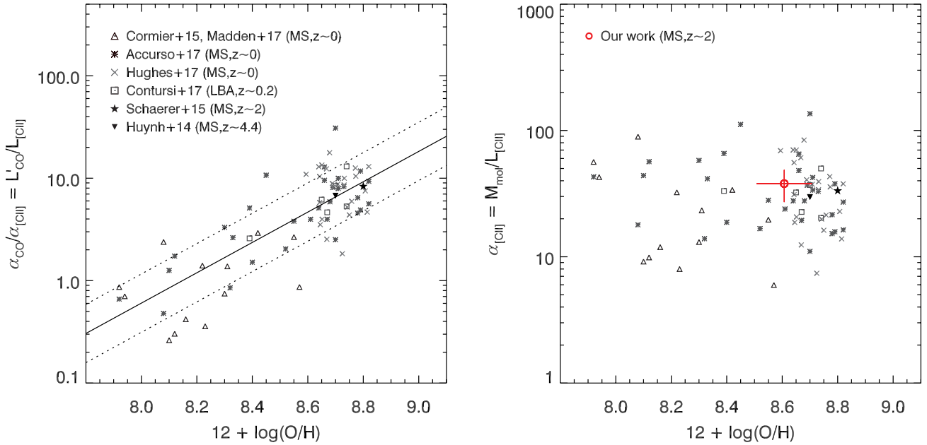
Figure 10. Metallicity dependence of \alpha_{\text{C II}} for multiple samples with available metallicity estimate, all homogenized to the Pettini & Pagel (2004) calibration using the parametrizations by Kewley & Ellison (2008). The symbols are the same as reported in Figure 6 caption and legend. Left panel: ratio of the CO and [C II] luminosity as a function of the galaxies gas phase metallicity. The linear fit of the two samples is reported (black solid line). Right panel: [C II]-to- \text{H}_2 conversion factor as a function of metallicity. The average measurement for our sample (red empty circle) is reported only in this panel since no CO measurements are available for our sources. The gas mass for our galaxies was estimated considering the integrated Schmidt-Kennicutt relation (see Section 2.4). We note that one of the galaxies by Cormier et al. (2015) is an outlier to the L_{\text{C II}} - M_{\text{mol}} relation (and therefore of the \alpha_{\text{C II}} - metallicity estimate) due to its very low [C II] luminosity with respect to the CO one. We kept this galaxy in the sample for consistency with the literature, although there might be some issues with its [C II] and/or CO measurements.
