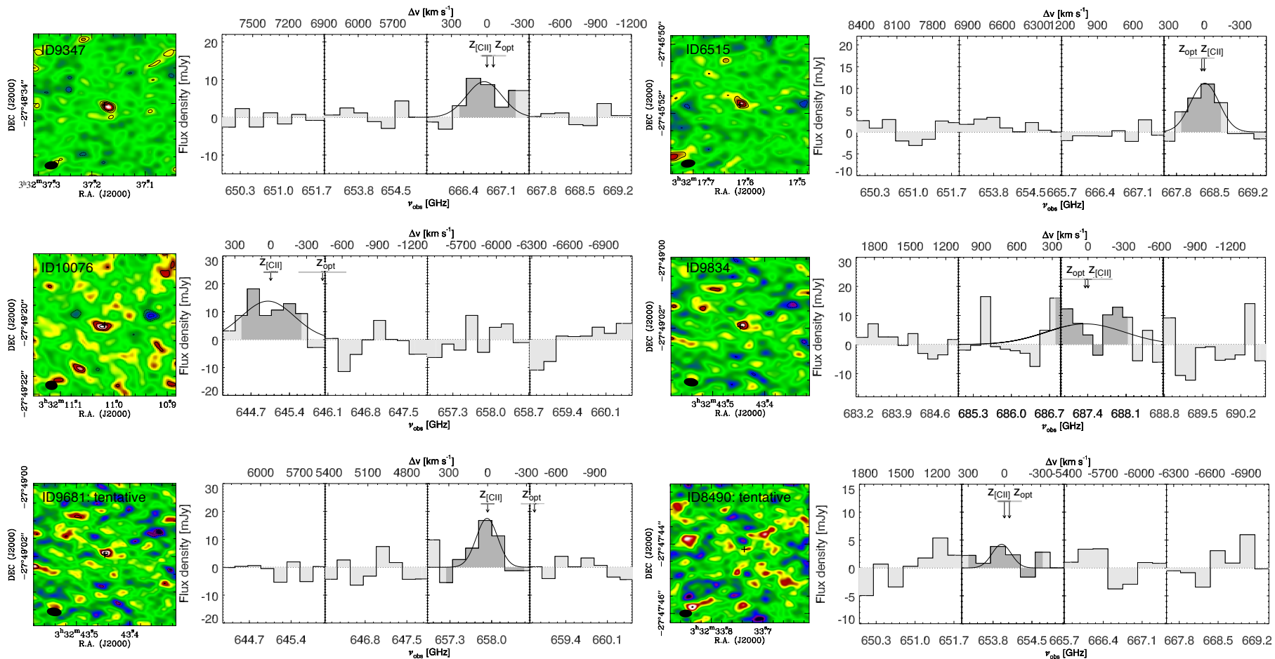
Figure 2. ALMA spectra of the [\text{C II}] detections of our sample. Left panels: ALMA 2D maps of the [\text{C II}] emission line. The black solid and dashed contours indicate respectively the positive and negative 3\sigma , 4\sigma , and 5\sigma levels. The beam is reported as the black filled ellipse. Each stamp has a size of 4'' \times 4'' . The black cross indicates the galaxy center, as estimated from the HST F160W imaging. Some tapering has been done for illustrative purposes, although we used the untapered maps for the analysis. Right panels: 1D spectra of the [\text{C II}] detected sources extracted using a PSF (notice that in this figure we did not scale the fluxes of the spectra extracted with PSF to match those obtained when using an exponential function with larger size as reported in Table 2). The dark grey shaded areas indicate the 1\text{-}\sigma velocity range over which the flux has been measured. The frequencies corresponding to the optical and [\text{C II}] redshifts are marked with arrows. The horizontal bars indicate the 1\sigma uncertainty associated to the optical (light gray) and [\text{C II}] (dark gray) redshift estimate. For illustrative purposes we also report the Gaussian fit of the emission lines: it was not used to estimate the line fluxes, but only as an alternative estimate of the galaxies' redshift (Section 2.3).
