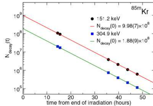
FIG. 11. The number of ^{85\text{m}}\text{Kr} decaying via \beta^- calculated from the \gamma photopeak at 151.2 keV [75.2(5)% intensity], and via IT calculated from the \gamma photopeak at 304.9 keV [14.0(3)% intensity]. The measured ratio is 0.188(9) in good agreement with the intensity ratio 0.186(4) in [49] (see Table II).
