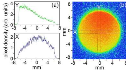
FIG. 4. (b) An auto-radiographic scan of the 13 mm diameter gold foil from the Kr irradiation above neutron production threshold. Colors indicate activity, decreasing from red to blue. (a) Profiles of a vertical (X) and horizontal (Y) slice of the scan. A vertical offset in neutron distribution (4.8(2) mm) is observed attributed to vertical steering of the proton beam. This offset is taken into account in the simulations.
