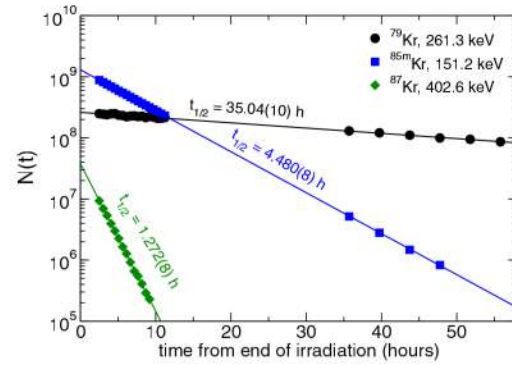
FIG. 10. Decay curves of ^{79}\text{Kr} , ^{85\text{m}}\text{Kr} , ^{87}\text{Kr} . The half-lives obtained from exponential fits of the curves (see text) are in good agreement with the adopted values in the literature (labeled in the figure).
