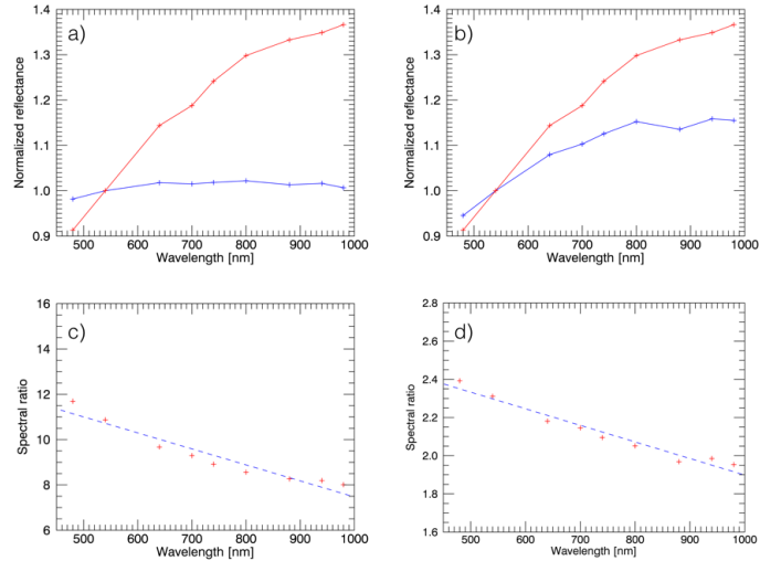
Fig. 11. a) and b) normalized reflectance spectra corresponding to different steps of a sublimation experiment using \mu m-sized H 2 O ice mixed with 5 wt.% basaltic airfall ash and 1 wt.% nanoparticle carbon as initial material. The red spectra in plots a) and b) are those of the final material at the end of the sublimation experiment. The blue spectrum in plot a) was acquired at the very beginning of the sublimation. The blue spectrum in plot b) was acquired about 10 h later. All spectra were normalized to their value of reflectance at 535.7 nm. c) and d) corresponding spectral ratios between the blue curves and red curves in plots a) and b) , respectively (crosses) and linear fit through these points (dashed lines).
