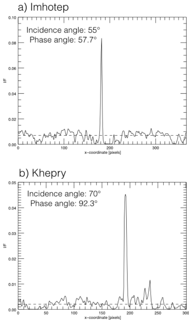
Fig. 6. Profiles of radiance factor I/F through two different bright features: a) bright field shown in Fig. 1a. b) Bright feature shown in Fig. 6a. The average incidence angles estimated from the DTM are 55^\circ and 70^\circ , respectively. This gives multiplication factors of 1.74 and 2.92, respectively, to calculate the reflectance factors, which reach about 0.13 in both cases over the brightest spots.
