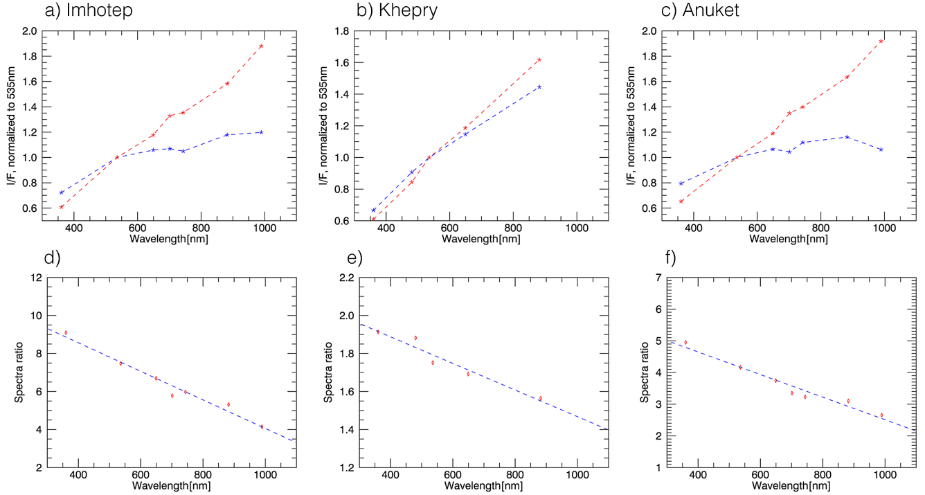
Fig. 9. a), b), and c) average normalized reflectance spectra of three different bright features (blue) and dark terrain nearby (red) for the examples shown in Figs. 7e, c, and a, respectively. Spectra of the bright features were averaged over a region of interest (ROI) of a few pixels defined inside the bright feature, avoiding its edges that are often affected by imperfect coregistration at the pixel scale. Spectra of the dark soil were averaged in a similar way over regions defined by avoiding all visible shadows in the image. All spectra were then normalized by their value of reflectance at 535.7 nm. d), e), and f) corresponding ratios between the average spectra of the bright feature and the average spectra of the dark soil (crosses) and linear fit through these points (dashed lines).
