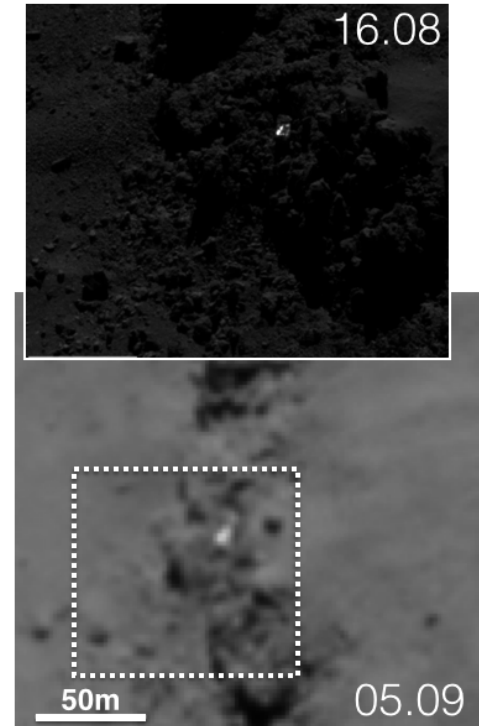
Fig. 5. Effect of the spatial resolution on the aspect of surface bright features. In both examples shown here, the surface shown at higher resolution allows resolving small meter-sized bright spots inside what looks like homogeneous bright regions at lower scale. As a result, the bright spots are much smaller and brighter than what could be inferred from the earlier lower resolution observation. a) Imhotep. Subset of OSIRIS NAC images: NAC_2014-08-16T19.59.14.556Z_ID30_1397549300_F22.IMG NAC_2014-09-30T20.44.47.569Z_ID30_1397549300_F22.IMG; b) Hatmehit. Subset of OSIRIS NAC images: NAC_2014-08-16T15.59.14.568Z_ID30_1397549500_F22.IMG NAC_2014-09-05T08.00.55.651Z_ID30_1397549500_F22.IMG.
