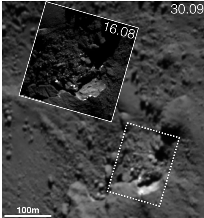
Fig. 5. Effect of the spatial resolution on the aspect of surface bright features. In both examples shown here, the surface shown at higher resolution allows resolving small meter-sized bright spots inside what looks like homogeneous bright regions at lower scale. As a result, the bright spots are much smaller and brighter than what could be inferred from the earlier lower resolution observation. a) Imhotep. Subset of OSIRIS NAC images: NAC_2014-08-16T19.59.14.556Z_ID30_1397549300_F22.IMG NAC_2014-09-30T20.44.47.569Z_ID30_1397549300_F22.IMG; b) Hatmehit. Subset of OSIRIS NAC images: NAC_2014-08-16T15.59.14.568Z_ID30_1397549500_F22.IMG NAC_2014-09-05T08.00.55.651Z_ID30_1397549500_F22.IMG.
