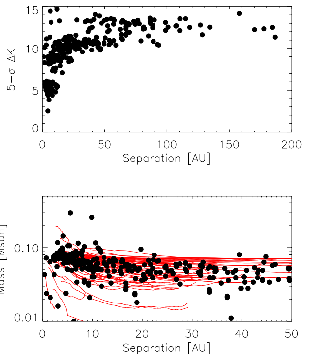
Fig. 7. Top: detection limits at 5\text{-}\sigma with respect to physical separation, for 0.12-0.24-0.5 and 1" angular separations and all stars included in this study (IRDIS only). Bottom: corresponding minimum mass and physical separation of each star in the sample, derived from IRDIS (black points) and IFS (red lines) detection limits.
