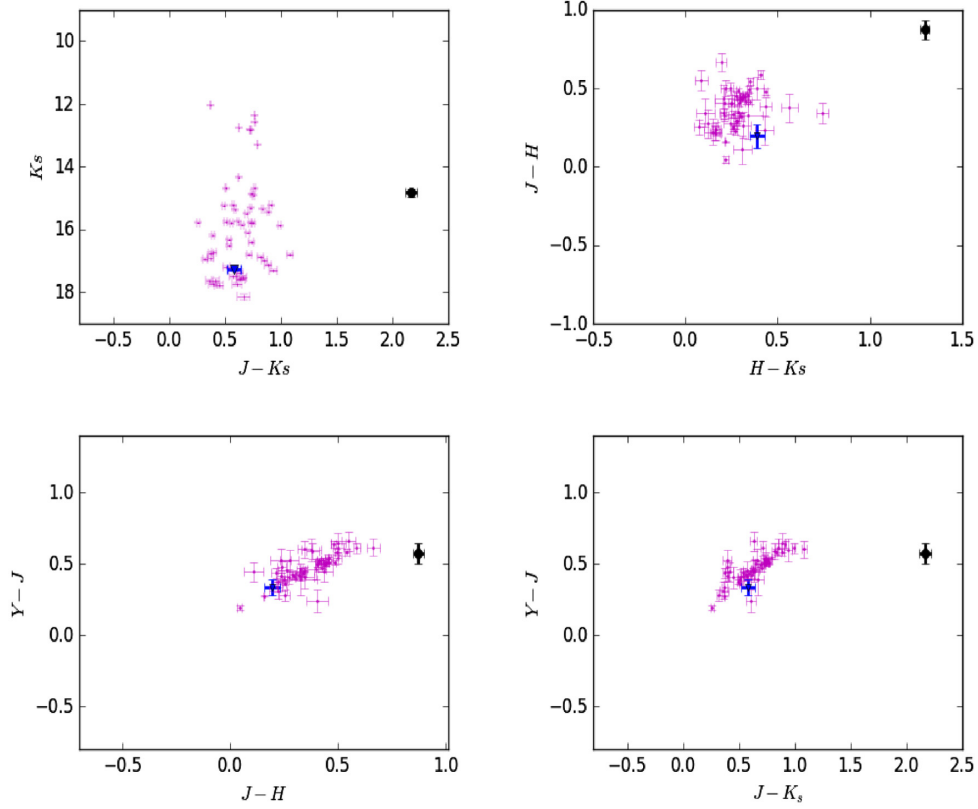
Figure 7. 5BZQJ1802–3940. (J - K_s) versus K_s CMD, (H - K_s) versus (J - H) , (J - H) versus (Y - J) , and (J - K_s) versus (Y - J) CCDs using near-IR data from the VVV survey. The symbols are represented as in Fig. 3.
