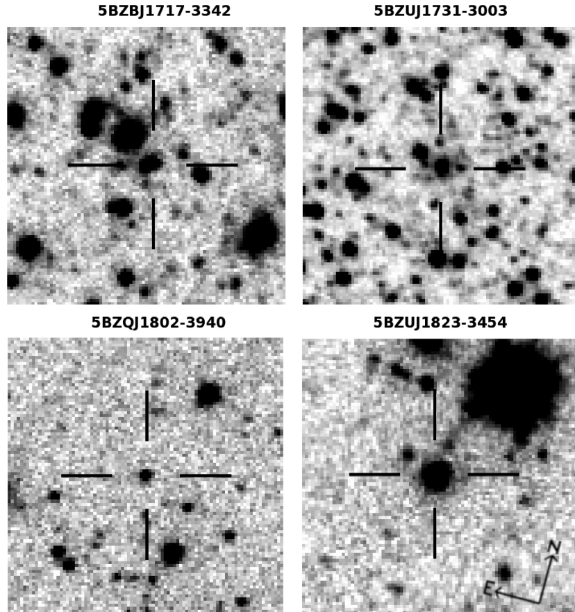
Figure 2. Stacked 0.5 arcmin \times 0.5 arcmin K_s images of the four blazars. The orientation is shown in the bottom right panel.
