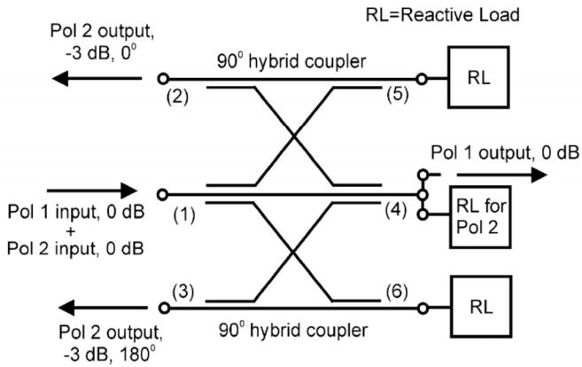
Fig. 2. Schematic representation of the ideal polarization splitting network (OMT) with forward coupling of Pol 1 from ports 1 to 4 and symmetric 3-dB backward coupling of Pol 2 from port 1 to ports 2 and 3. The structure consists of two 90° hybrid couplers with reactively loaded (RL) outputs. Port 1 is in common to the two hybrids. Signals at ports 2 and 3, 180° out-of-phase, are re-combined by a 180° power combiner.
