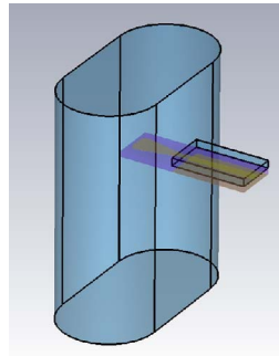
Fig. 4. Parallel H-plane waveguide-to-microstrip transitions employed in the dual polarization receiver module (left). Smith chart with simulation results of the transition across 75-116 GHz.
