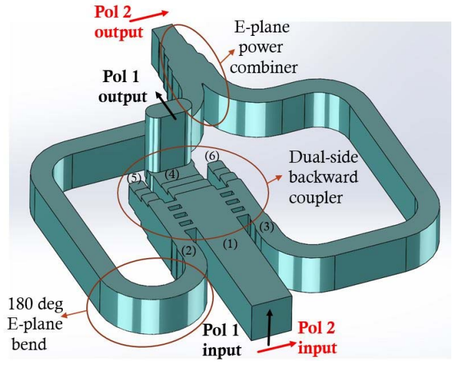
Fig. 3. 3D view of the OMT passive part showing the polarization splitting dual-side backward coupler, the two 180 deg and 90 deg E-plane bends, the E-plane power combiner, and the 90 deg E-plane bend transition. Numbers (1)-(6) inside or close the waveguides of the backward coupling structure refer to the port numbering adopted in the schematic of Fig. 2.
