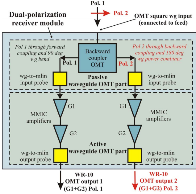
Fig. 1. Block diagram of dual-polarization receiver module based on a passive OMT part and on an active part integrating MMIC LNAs.
