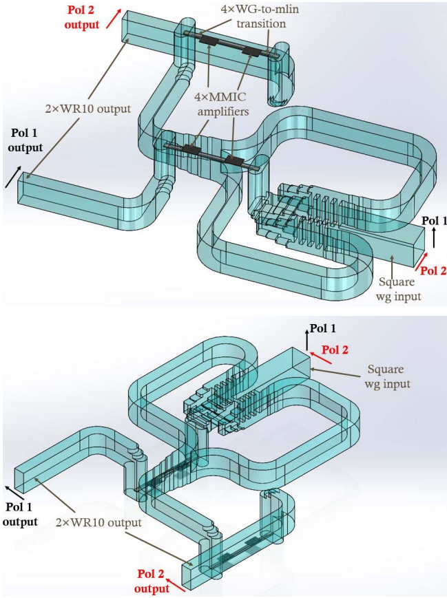
Fig. 5. Two different 3D views of the inner part of the dual-polarization receiver module showing the passive and active waveguide OMT parts, including the waveguide circuitries and the MMIC amplifiers.
