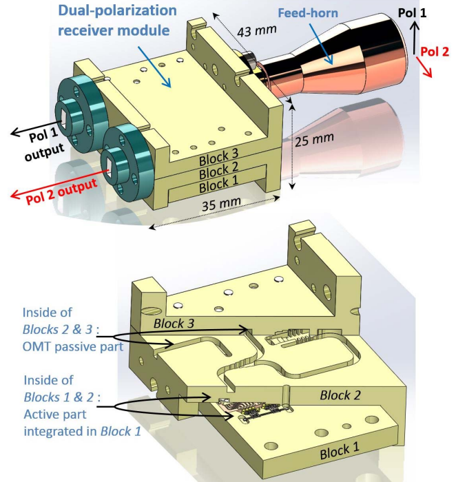
Fig. 6. 3D view of the dual-polarization receiver module. Top: fully assembled module with a feed-horn mounted at its input and two UG387 flanges mounted at its output to demonstrate its mechanical compatibility with external components. Bottom: cross-cut of the module showing the inner waveguide circuitry of the backward-coupler OMT implemented in Blocks 2 & 3 and the active part incorporated in Block 1.
