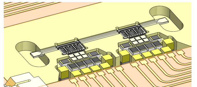
Fig. 7. 3D view of Block 1 (top) showing the packaging details of the MMICs with the waveguide-to-microstrip transitions and the bias circuitries, which include discrete capacitors and resistors (bottom).
