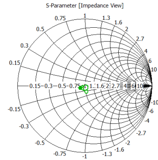
Fig. 4. Parallel H-plane waveguide-to-microstrip transitions employed in the dual polarization receiver module (left). Smith chart with simulation results of the transition across 75-116 GHz.
