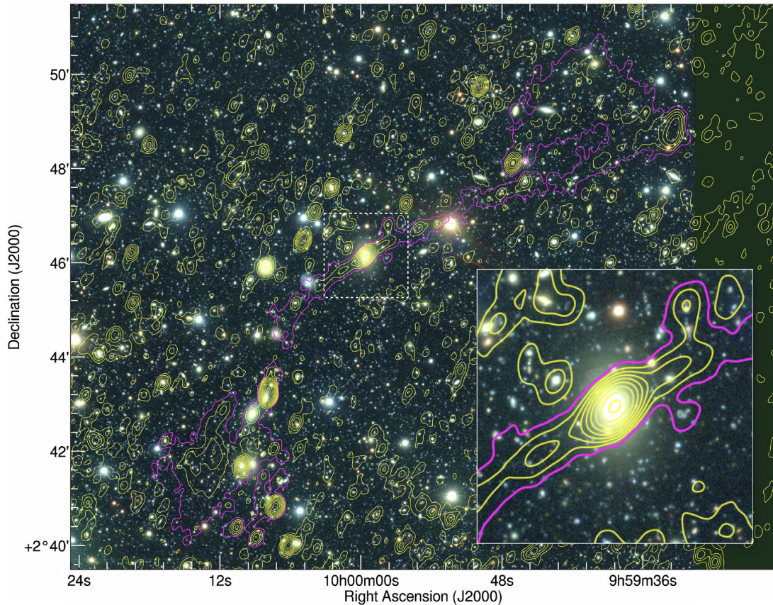
Figure 2. GRG1 as seen in MIGHTEE (yellow contours), overlaid on a composite optical image of HSC g , r , and i bands. Contours are shown at intervals of 30\sqrt{3} \mu\text{Jy beam}^{-1} , where n = 0, 1, 2, \dots, 20 . The lowest contour level is 7 \mu\text{Jy beam}^{-1} and is shown in magenta, as in Fig. 1, to highlight the full extent of the GRG. The inset shows an enlargement of the core area, where the host galaxy can be seen.
