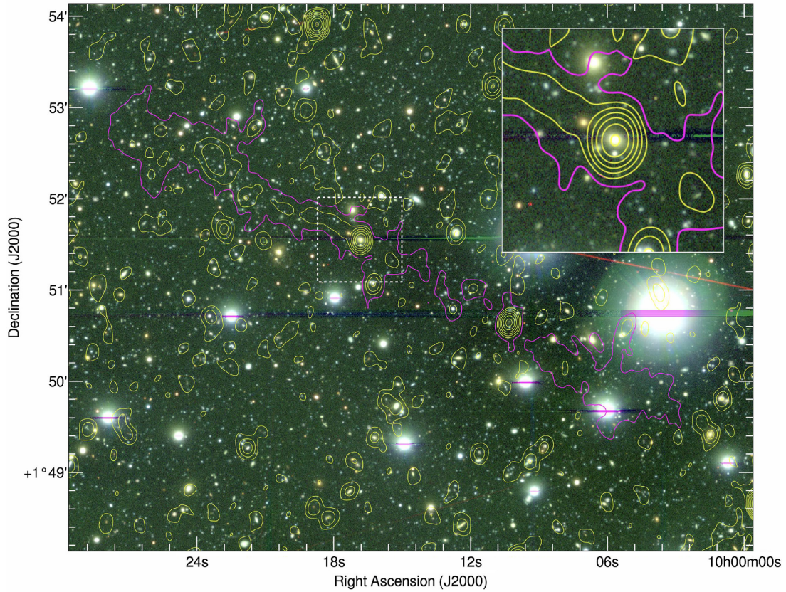
Figure 6. GRG2 as seen in MIGHTEE (yellow contours), overlaid on a composite optical image of HSC g , r , and i bands. Contours are shown at intervals of 20\sqrt{3} \mu\text{Jy beam}^{-1} , where n = 0, 1, 2, \dots, 20 . The lowest contour level is 5 \mu\text{Jy beam}^{-1} and is shown in magenta, as in Fig. 1, to highlight the full extent of the GRG. The inset shows an enlargement of the core area.
