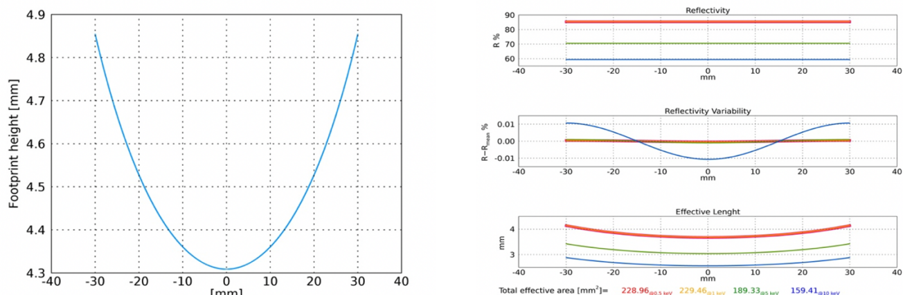
Figura 8 The same of previous figure in the case of a beam with parallel short sides.
