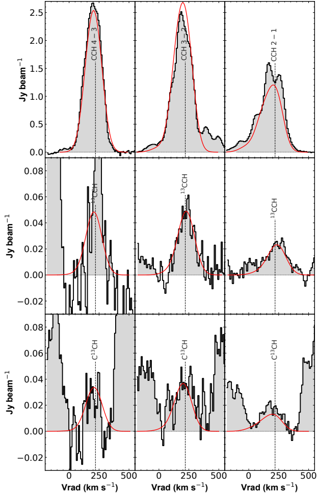
Fig. 14. Spectral features of the J = 4 - 3 (left), 3 - 2 (center) and 2 - 1 (right) transitions from three of the isotopologues of CCH detected in the survey. Red curves show the LTE model best fits. Contributions by other species is almost negligible for most transitions according to the global LTE model from the full survey (see Sect. 4.3.2). However we note that the observed profile of ^{13}\text{CCH } 4 - 3 , not following the CCH LTE model and not accounted for by emission from other species, was not used in the fit.
