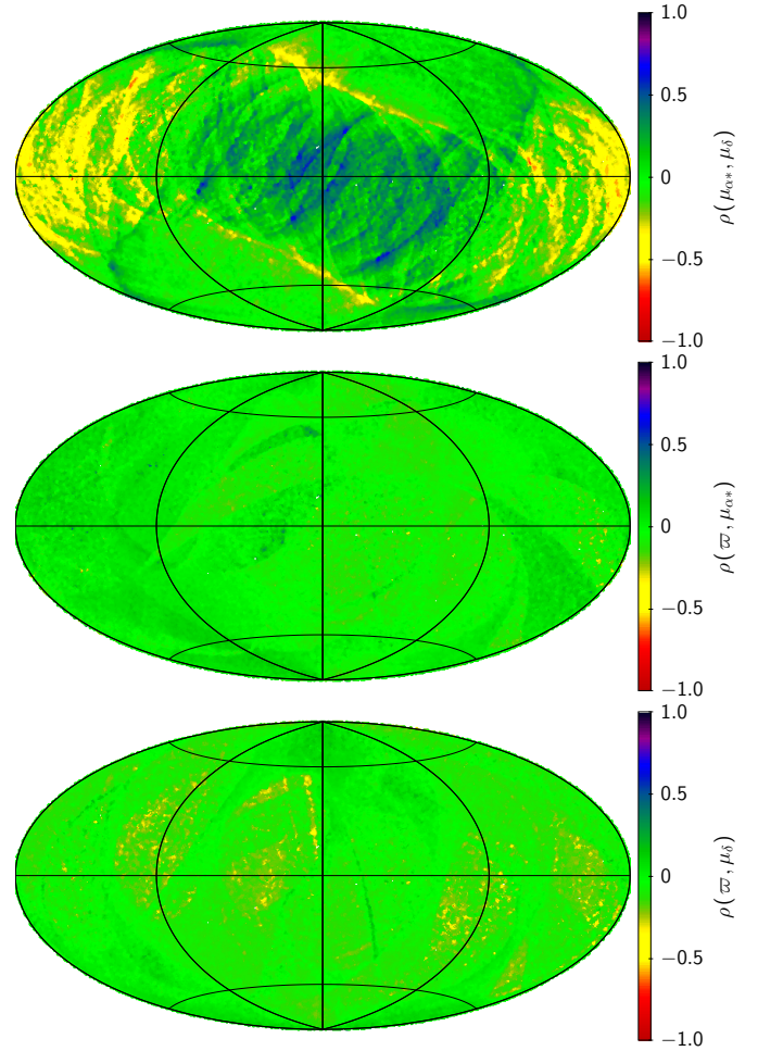
Fig. 15. Median correlations between parallaxes \varpi and proper motions \mu_{\alpha}, \mu_{\delta} in HIP-TGAS.
