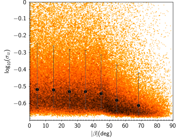
Fig. 12. Logarithm of the parallax errors (mas) in function of ecliptic latitude for the HIPPARCOS subsample in TGAS. The points show the medians, while the error bars show the 10th and the 90th percentiles of the distribution.
