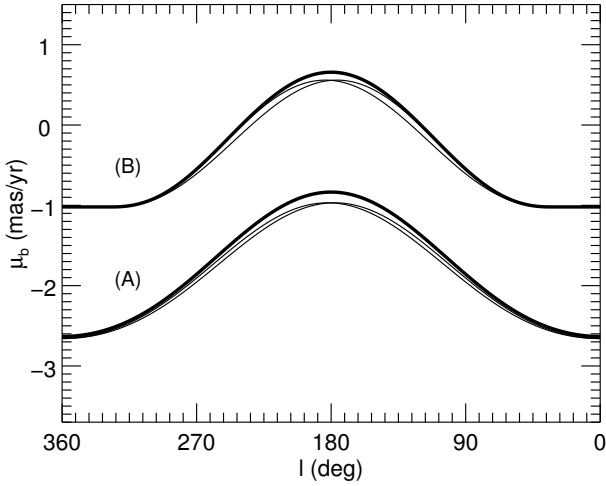
Fig. 2. According to the warp model, the true \mu_b in the Galactic plane as a function of Galactic longitude at heliocentric distances of 0.5 kpc (A) and 1.5 kpc (B). For each set of curves, the thick line represents the case with warp phase \phi_w = 0^\circ and the two thin curves show \phi_w = \pm 20^\circ .
