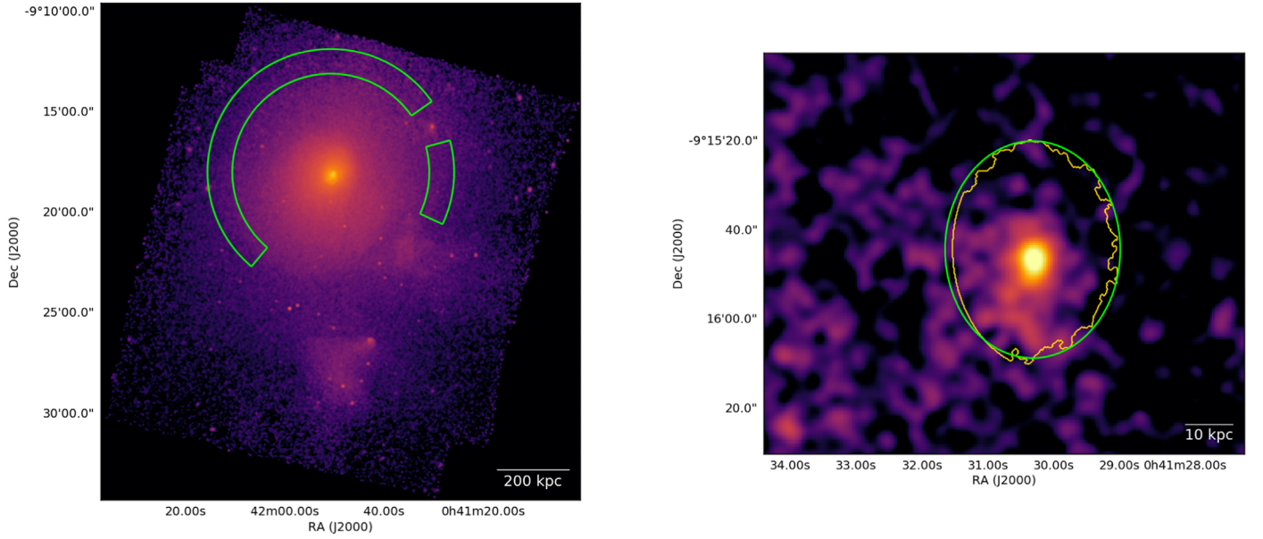
Figure 3. Left panel: exposure-corrected mosaic of the cluster A85 in the 0.5–2.0 keV; the region used to extract spectra from the ICM is shown in green. Right panel: zoomed-in image of JO201; the region used to extract spectra from the stellar disk mask is represented in green, while the contour of the stellar disk (Gullieuszk et al. 2020) used as reference is shown in gold.
