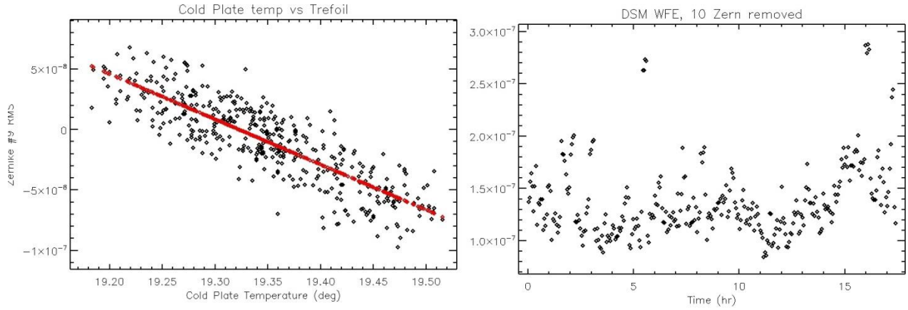
Figure 23 Left panel: Zernike Z6 trefoil versus cold plate temperature; right panel: WFE (rms) during the test, after the correction of 10 Zernike modes to compensate for thermo-mechanical drifts.
