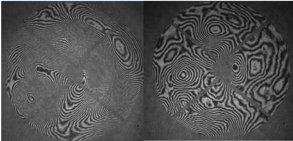
Figure 2 First image of the DSM thin shell as seen by the interferometer on ASSIST.
