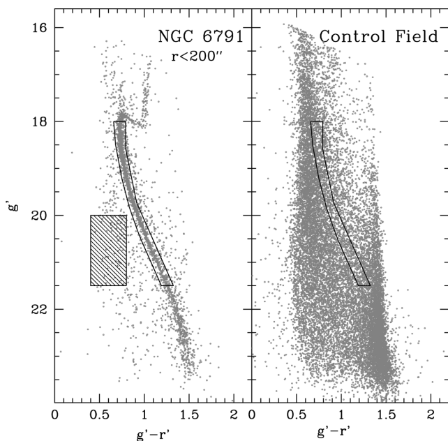
Figure 2. (g', g' - r') CMDs of the innermost region of NGC 6791 (left-hand panel) and of the control field (right-hand panel). The black box along the MS of NGC 6791 encloses the region in the CMD where CP stars have been selected. The shaded area defines the region where fiducial Galactic disc MS stars have been selected.
