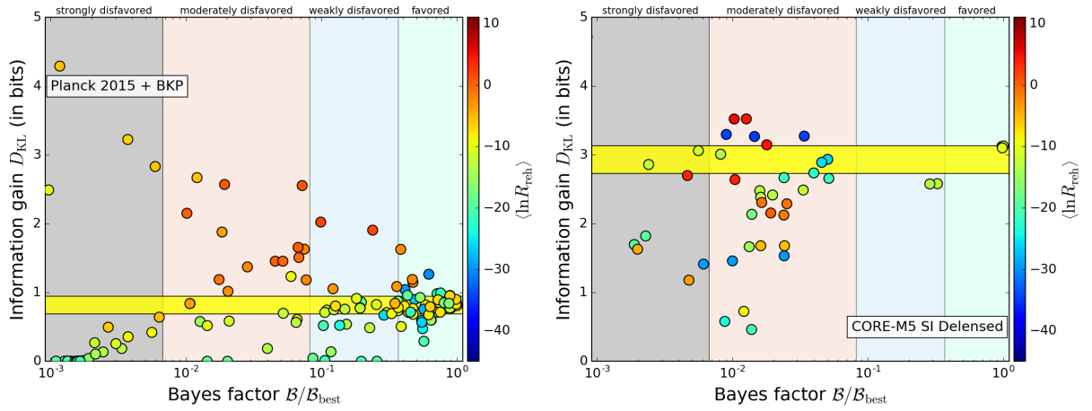
Figure 16: Information gain on reheating measured by the Kullback-Leibler divergence D_{\text{KL}} (in bits) on the reheating parameter \ln R_{\text{reh}} for Planck 2015 + BKP joint cross-correlation [54] (left panel, results taken from Ref. [228]) and for CORE-M5 if SI is the fiducial model, as a function of the Bayesian evidence normalized to the best model. Each circle represents one model and the x -axis is divided into Jeffreys categories. The circle color traces the mean value of the reheating parameter \ln R_{\text{reh}} . The yellow band represents the 1\sigma deviation around the mean value for D_{\text{KL}} .
