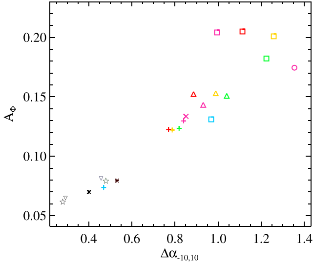
Figure 11. Plot of— the area A_\phi under the MFS and above f=1.5 versus \Delta\alpha_{-10,10} for maps for which both quantities can be derived. The symbols are the same introduced in the legend of Fig. 8.
