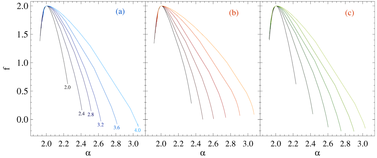
Figure 7. MFS of the fBm reference images reported in Fig. A1, grouped by image phase distribution (cases ‘A’, ‘B’, and ‘C’ in left-hand, middle, and right-hand panel, respectively). A different colour shade, from the darkest to the lightest, is used for indicating images with the power spectrum exponent \beta ranging from 2 to 4 in steps of 0.4.
