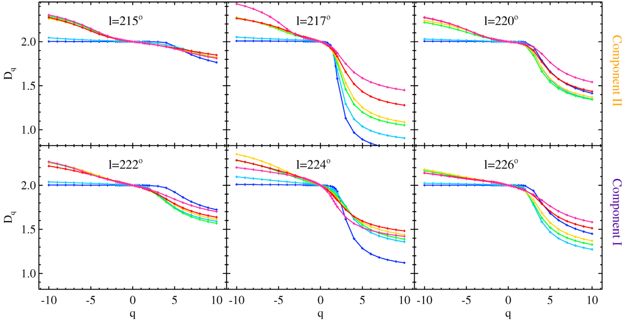
Figure 15. Generalized fractal dimension D_q versus order q for the Hi-GAL maps analysed in this work, ordered by tile and colour-coded as in Fig. 5.
