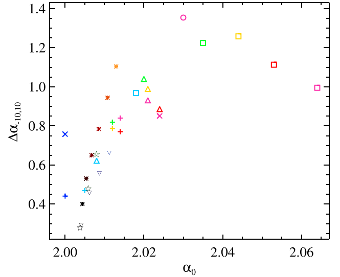
Figure 10. Plot of the MFS ‘amplitude’ \Delta\alpha_{-10,10} versus the peak position \alpha_0 for the maps studied in this work for which a reliable \alpha values in the 10 \leq q \leq 10 range was derived. Data corresponding to the three turbulent ISM simulations with available \Delta\alpha_{-10,10} (see Table 3) are all located at \alpha_0 > 2.1 and \Delta\alpha_{-10,10} > 2.2 and are not displayed here not to overly compress the plot. The symbols are the same introduced in the legend of Fig. 8.
