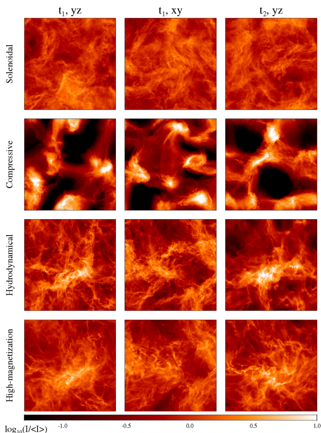
Figure 2. Column density maps obtained by projecting three-dimensional simulated density fields selected in the STARFORMAT archive. The rows, from top to bottom, correspond to four different scenarios, namely ‘solenoidal forcing’, ‘compressive forcing’, ‘quasi-hydrodynamical’, and ‘high-magnetization’, respectively (see the text). The images in the upper two rows are composed by 256 \times 256 pixels, while those in the lower two rows are composed by 2048 \times 2048 pixels, see Table 1. In each column a different combination of epoch and projection direction is displayed: the assignment of yz and xy plane denominations follows the notation used in STARFORMAT, used here only to indicate that the two planes are orthogonal. With t_1 and t_2 we do not indicate, in general, the same time for all the four scenarios, but only two different epochs such that t_1 < t_2 ; they coincide for the first and the second scenario only. Further details of the simulations are reported in the text. Maps are represented here by arbitrarily normalizing their values by the map average \langle I \rangle , and rendered through a logarithmic scale, choosing an image saturation level of \log_{10}(10\langle I \rangle) , to better appreciate the low-density fluctuations.
