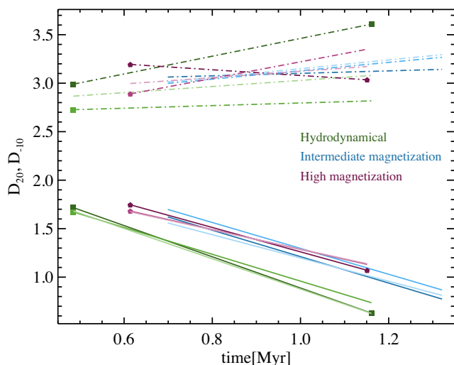
Figure B2. Evolution in time of the fractal dimensions D_{20} (solid lines, lower part of the plot) and D_{-10} (dot-dashed lines, upper part) for the ‘quasi-hydrodynamical’ (green), ‘intermediate magnetization’ (blue), and ‘high-magnetization’ (pink) numerical simulations of column density, respectively. All three projections are taken into account (dark, intermediate, and lighter colour for yz , xy , and xz , respectively). Only two time-steps are available, with the two times depending on the scenario (cf. Section 2.2). As in Fig. B1, the values of D_{20} and D_{-10} already calculated and shown in Section 4.3 for particular combinations of scenarios and projection directions are marked with symbols (assigned as in Fig. 8).
