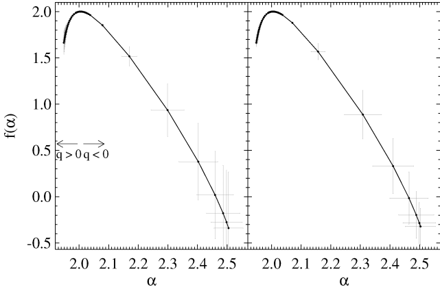
Figure 4. Left: MFS of the same fBm reference image used to build Fig. 3, obtained through equations (8) and (9), exploring the range of orders -10 \leq q \leq 20 , in steps of \Delta q = 1 (but \Delta q = 0.2 in -2 \leq q \leq 2 ). The error bars are displayed as grey crosses for each point, to give an idea of the typical uncertainties affecting the MFS estimation. Right: The same as in the left-hand panel, but computed through equations (13) and (14).
