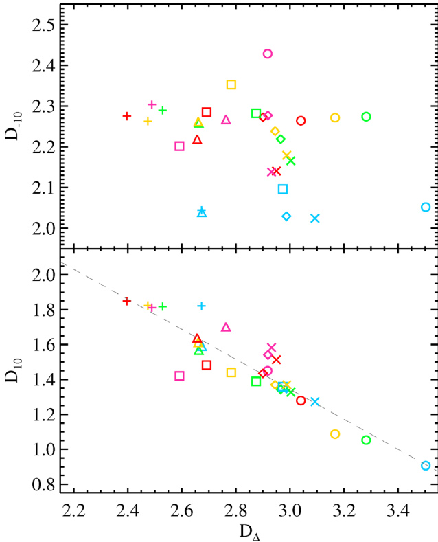
Figure 16. Plot of the fractal dimensions of order q = -10 (top panel) and 10 (bottom panel) versus the mono-fractal dimension D_\Delta estimated through the \Delta -variance technique (see Appendix C) for the six Hi-GAL fields studied in this paper. Symbols and colours are the same coded in Fig. 8, with the addition of the \ell 226 maps, indicated with an asterisk. The 70\ \mu\text{m} maps are not shown, being D_\Delta unreliable for these maps (see Paper I).
