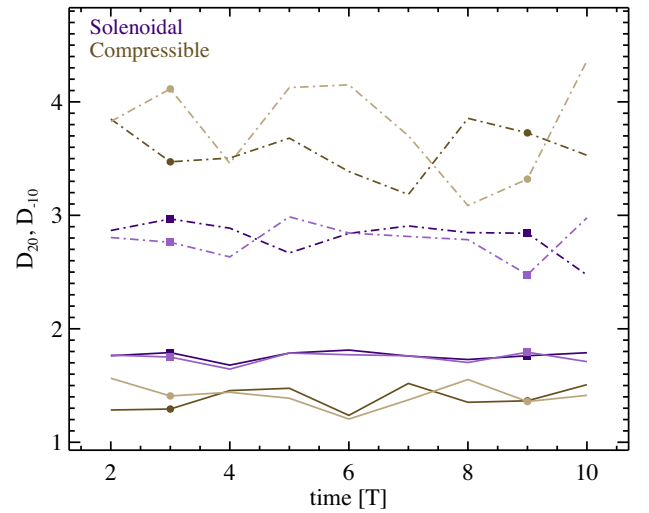
Figure B1. Evolution in time of the fractal dimensions D_{20} (solid lines, lower part of the plot) and D_{-10} (dot-dashed lines, upper part) for the ‘solenoidal forcing’ (purple) and ‘compressive forcing’ (brown) numerical simulations of column density, respectively. The two projections yz and xy (see Section 2.2) are taken into account (darker and lighter colour, respectively). The time is in units of T (see Section 2.2), and the values of D_{20} and D_{-10} for T=3 and 9 are marked with symbols (assigned as in Fig. 8), as they coincide with those already calculated and discussed in Section 4.3.
