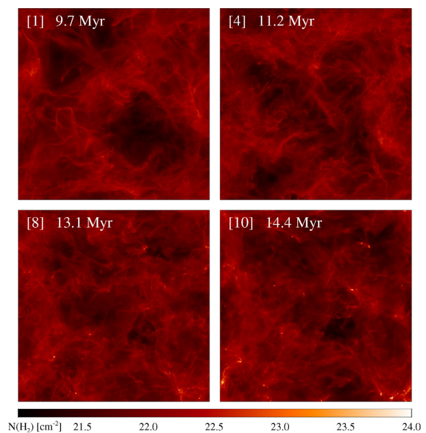
Figure B3. Four (out of 10) examples of column density snapshots obtained for this paper similarly to Hennebelle (2018). The number of the snapshot and the corresponding time are overwritten in white in each panel. In particular, the initial (top left) and final (bottom right) snapshots were chosen and displayed, and the first after the gravity is switched on (top right). Maps are in decimal logarithm of column density (in \text{cm}^{-2} ). The bottom colour bar applies to all maps, and to improve the rendering of relatively faint structures, it saturates at a value smaller than the maximum reached in the bottom right panel, namely \sim 25.2 .
