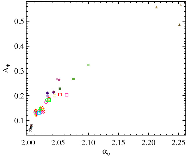
Figure 12. Plot of the area A_\phi under the MFS and above f=1.5 versus the peak position \alpha_0 for maps for which A_\phi can be derived. The symbols are the same introduced in the legend of Fig. 8.
