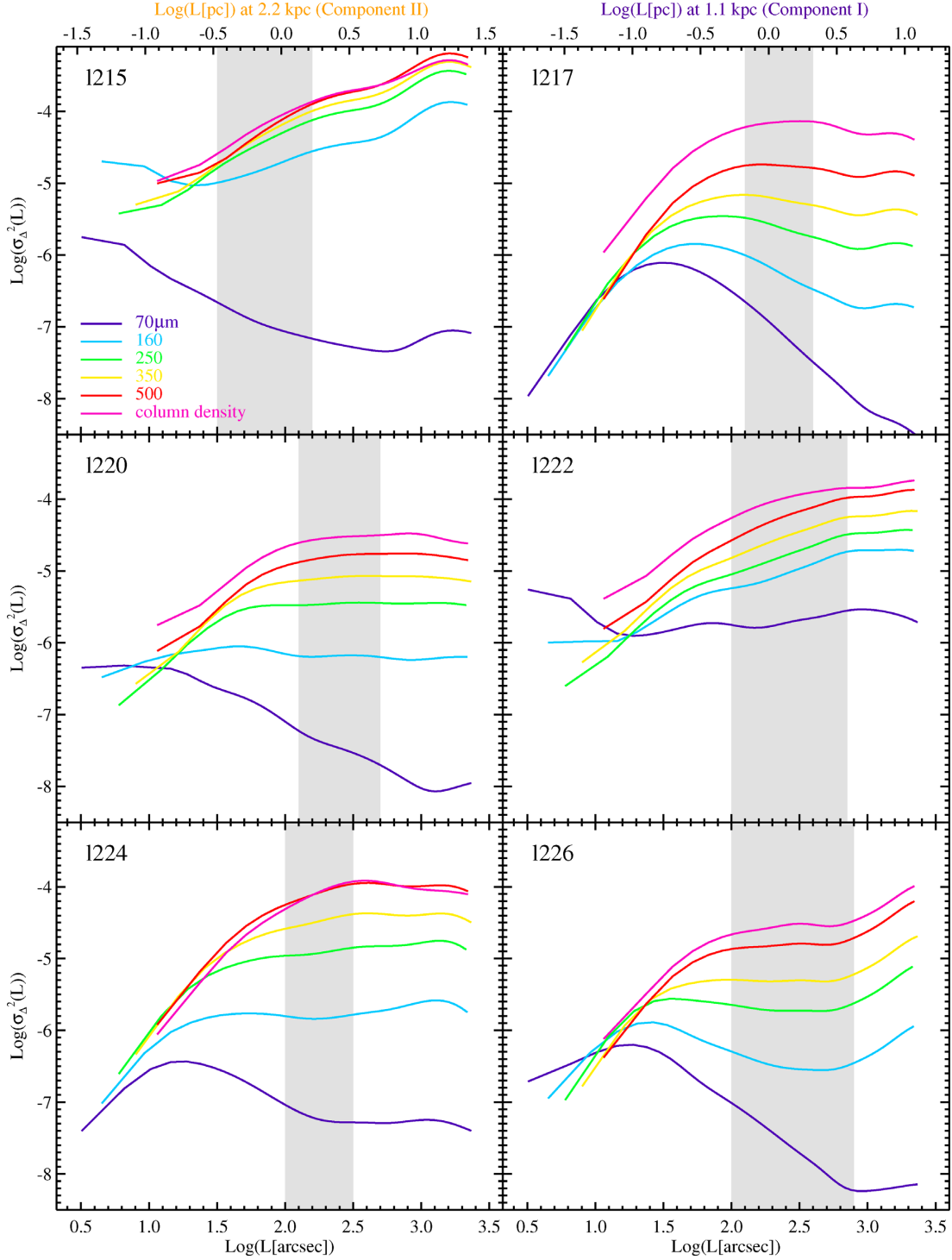
Figure C1. \Delta -variance curves of the maps shown in Fig. 1 using the same tile naming and band-colour encoding (this figure is similar to fig. 4 of Paper I). Tiles associated with velocity component II are in the left-hand panels, those associated with component I are in the right-hand panels (for reference, the spatial scales corresponding to angular scales at the distances of the two components are reported on the top axis of the two upper panels, respectively). We use the same axis ranges in all panels to allow a direct comparison of the slopes. The inertial range is highlighted as a grey area in each panel. The corresponding linear slopes are transformed in power spectrum slopes (see the text) are reported in Table C1.
