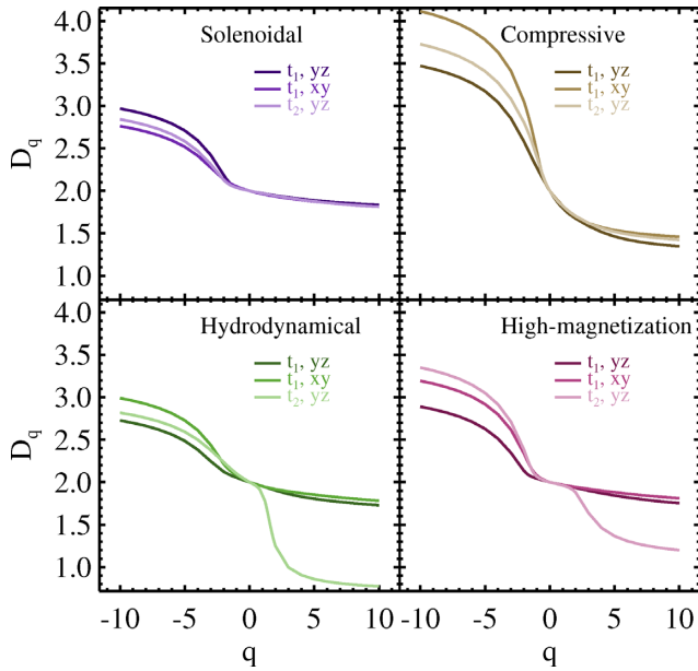
Figure 17. Generalized fractal dimension D_q versus order q for the column density maps produced by the numerical simulations analysed in this work, arranged by model and colour-coded as in Fig. 6.
