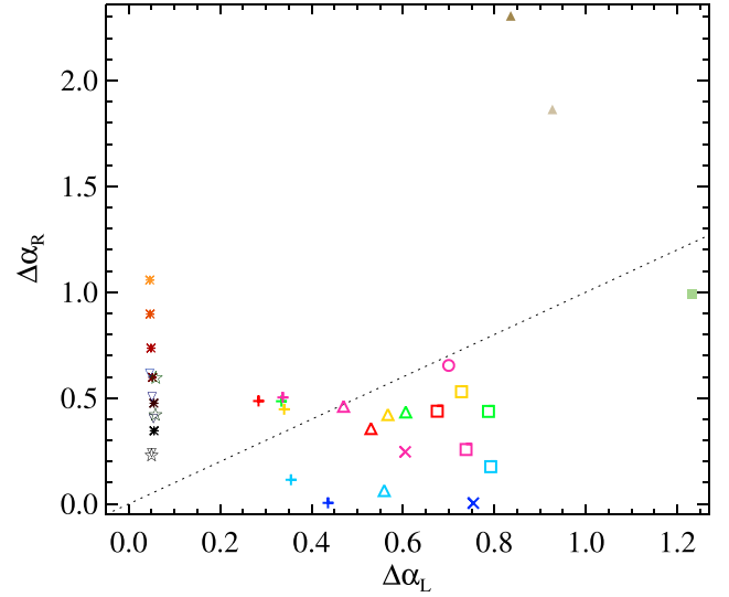
Figure 13. Plot of the MFS left versus right tail amplitude for maps for which it is possible to derive both quantities. The symbols are the same introduced in the legend of Fig. 8. The dotted line represents the bisector, to facilitate the distinction between left-skewed (below the line) and right-skewed (above the line) MFSs, respectively.
