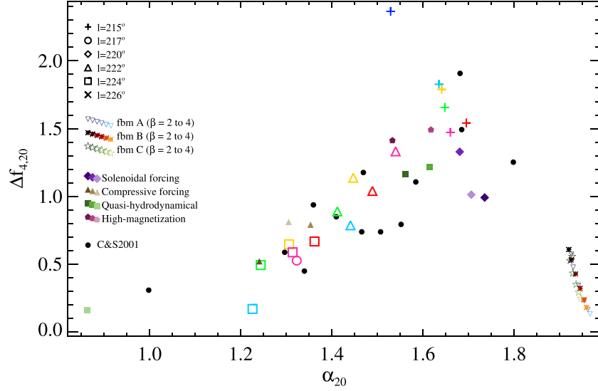
Figure 8. Plot of ‘dimensional diversity’, expressed by \Delta f_{4,20} \equiv f(q=4) - f(q=20) , versus the smallest computed value of the singularity strength \alpha_{20} \equiv \alpha(q=20) . Such quantities are available only for Hi-GAL maps with q_c^+ \geq 20 . The correspondence of symbols and colours with tiles and bands, respectively, is explained in the legend; the symbol for the tile \ell 226 , although not present in the plot, is introduced since the convention established here is used also in other following figures. Points representing the 12 cloud simulations and the 18 fBm images analysed in this work are plotted as well (symbols are explained in the legend). Furthermore, the positions of the 18 fBm reference images (located close to the bottom right corner of the diagram) are represented with smaller symbols, using colour scales (different for the ‘A’, ‘B’, and ‘C’ cases) to identify the different explored values of \beta . Finally, for comparison, points taken from fig. 8 of Chappell & Scalco (2001) and representing multifractal features of their IRAS -based column density maps of 13 nearby ( d \leq 160 pc) star-forming regions are reported as filled black circles (‘C&S2001’, in the legend).
