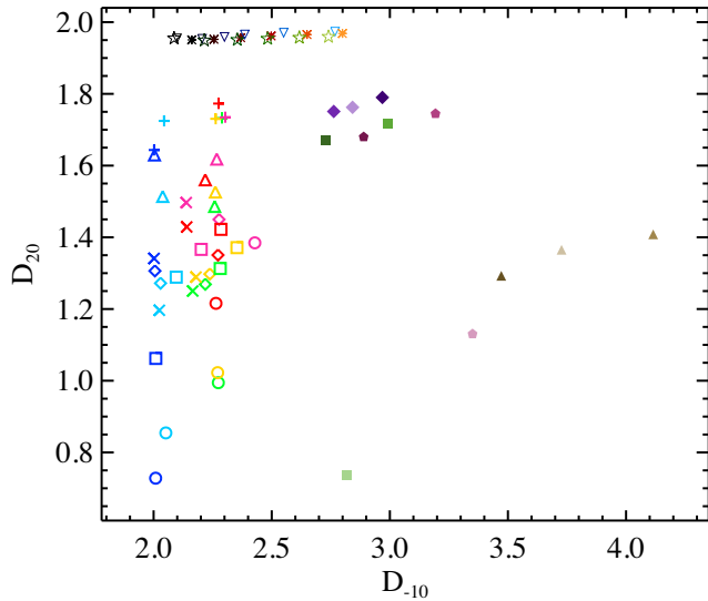
Figure 19. Fractal dimension of order q = 20 versus the one of order q = -10 for all the maps analysed in this paper. Symbols and colours are the same introduced in Fig. 8.
