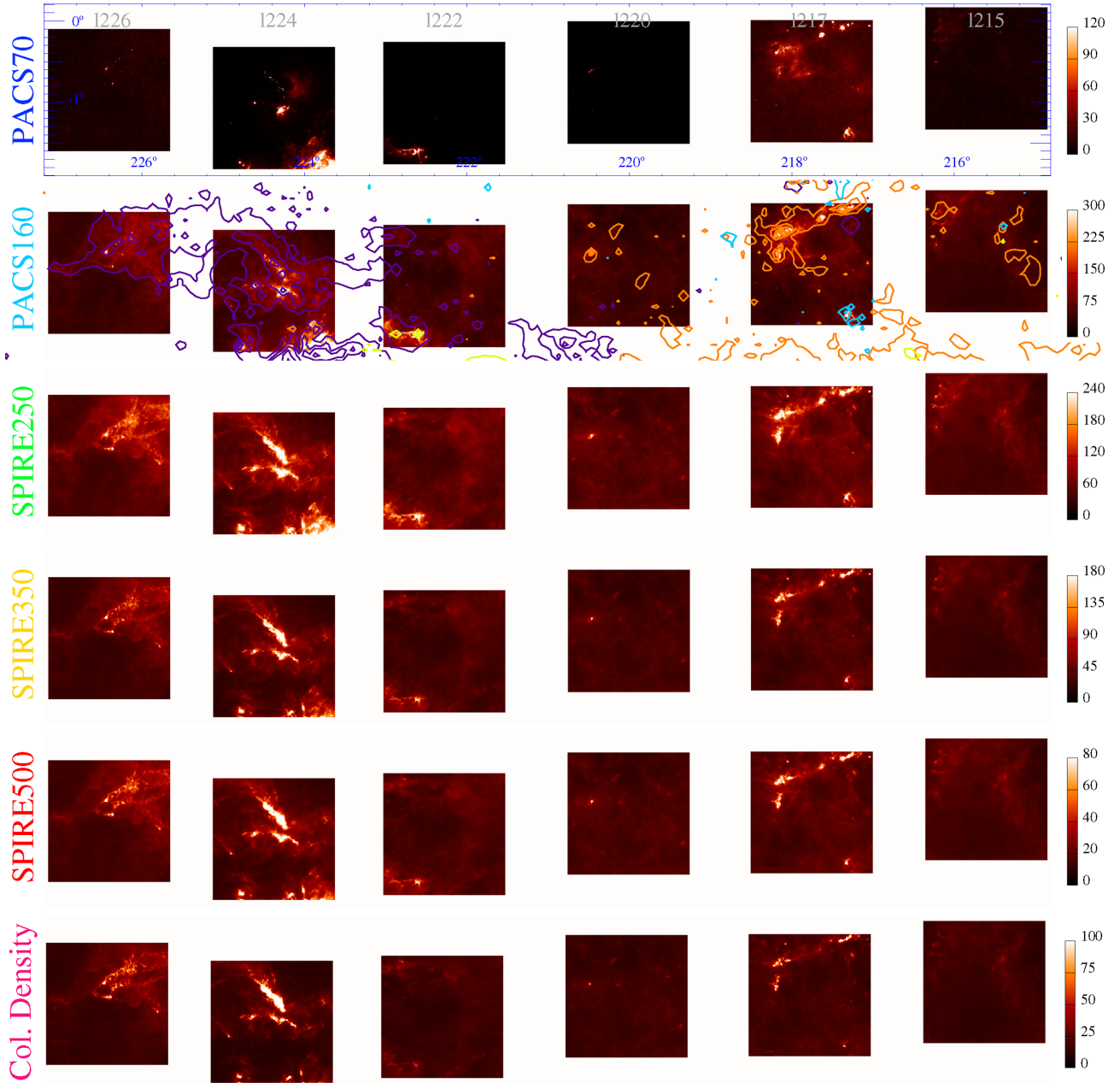
Figure 1. Each row shows the six Hi-GAL fields investigated in this paper. The instrument/band combination is specified in each row, adopting the colour convention that is used throughout the rest of the paper, namely blue: 70 \mu\text{m} , cyan: 160 \mu\text{m} , green: 250 \mu\text{m} , yellow: 350 \mu\text{m} , red: 500 \mu\text{m} , magenta: column density. The colour scales are linear; we preferred this choice with respect to the logarithmic scale to show the actual dynamics of the maps processed in this paper. The units are \text{MJy sr}^{-1} for the PACS and SPIRE maps, and 10^{20} \text{ cm}^{-2} for the column density ones. The tile names and Galactic coordinate grid are displayed in the row of 70 \mu\text{m} images (longitude on the horizontal axis and latitude on the vertical axis). Notice that the frame displacement is a real effect due to the choice of square area cut from each original tile. The CO(1–0) contour levels of Elia et al. (2013) are overplotted on the row of 160 \mu\text{m} images. The contours start from 5 \text{K km s}^{-1} and are in steps of 15 \text{K km s}^{-1} . Velocity components I, II, III, and IV (see the text) are represented with purple, orange, yellow, and cyan contours, respectively.
