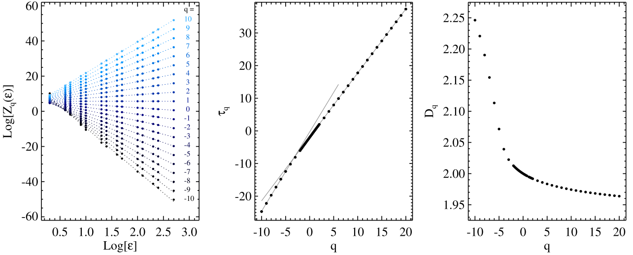
Figure 3. Example of derivation of the generalized fractal dimensions for a test 1000 \times 1000 pixel fBm image (see Section 2.3), in this case the one of type ‘C’ and \beta = 2.4 shown in Fig. A1. Left: logarithm of the partition functions Z_q(\epsilon) versus the logarithm of the integer scales \epsilon between 1 and 500 pixels for each integer value of the parameter q between -10 and 10 (in this range, different shades of blue, from the darkest to the lightest, respectively, are used for each different q ). The linear fit is shown as a dashed line of the same colour of the corresponding Z_q function (cf. equation 5). The functions for orders q > 10 and non-integer orders in the range -2 < q < 2 , although computed, are not shown here for the sake of clarity. Middle: scaling exponents \tau_q of the partition function, obtained through the linear fit shown in the left-hand panel as a function of q . To highlight the different slopes at negative and positive orders, the linear fit of the \tau_q versus q in the two the regions q < -3 and q > 3 , is shown by means of two grey lines. Right: generalized fractal dimension set, derived through equation (7), as a function of q , except for the case q = 1 , not contemplated by equation (7).
