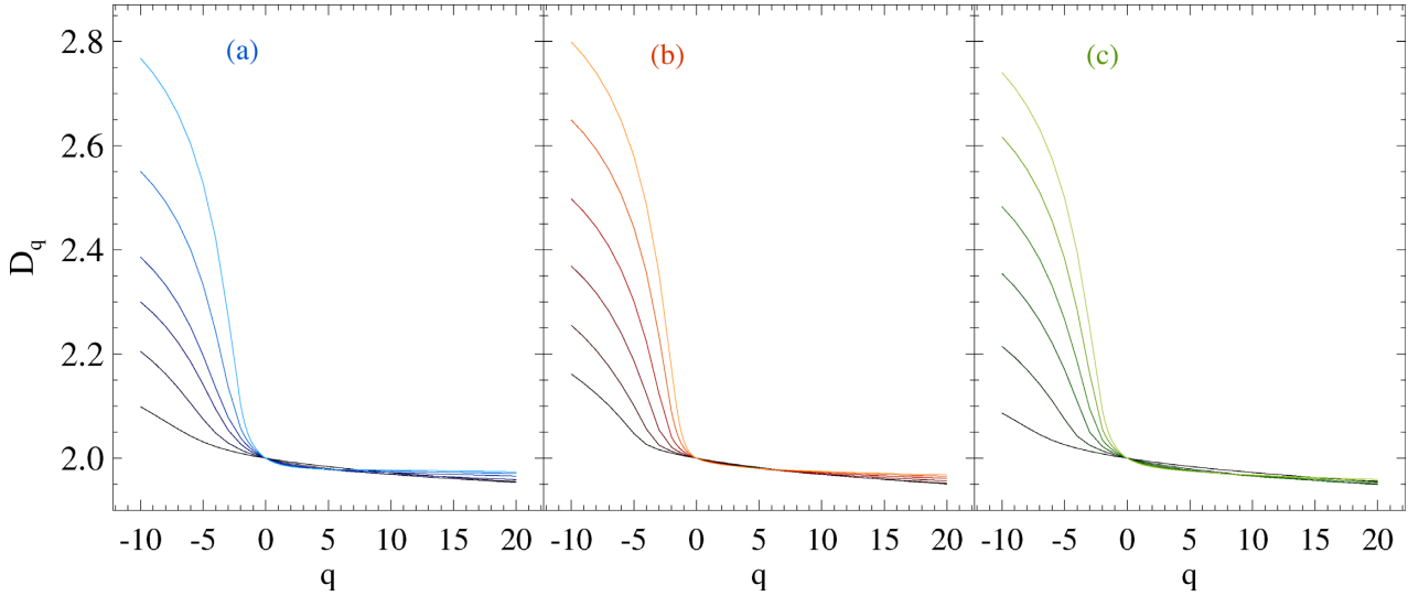
Figure 18. Generalized fractal dimension D_q versus order q for the fBm images analysed in this work, grouped by common phase distribution and colour-coded as in Fig. 4 (from dark to light as the power spectrum exponent \beta increases from 2 to 4 in steps of 0.4).
