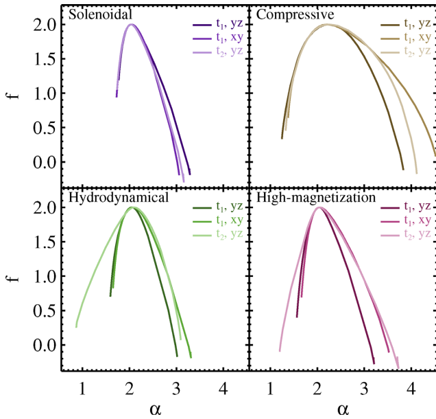
Figure 6. MFS of the column density maps obtained from simulations, shown in Fig. 2. In each panel the model, the projection plane, and the epoch of the simulation are specified for each displayed MFS. The range of \alpha on the horizontal axis is chosen to optimize the plot of the represented MFS, and for this reason a visual comparison with the plots in Fig. 5 (set according to the same criterion) cannot be performed directly.
