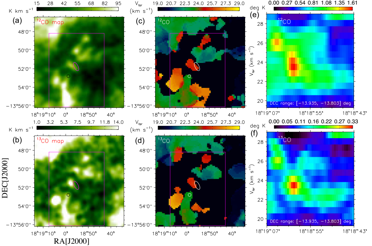
Figure 7. (a) FUGIN ^{12}\text{CO}(J = 1-0) integrated intensity map (at [19.275, 27.725] \text{ km s}^{-1} ). (b) FUGIN ^{13}\text{CO}(J = 1-0) integrated intensity map. (c) The line-of-sight intensity weighted velocity map of the FUGIN ^{12}\text{CO}(J = 1-0) emission. (d) FUGIN ^{13}\text{CO}(J = 1-0) intensity weighted velocity map. (e) Position (or right ascension)-velocity diagram of the FUGIN ^{12}\text{CO}(J = 1-0) emission. The molecular emission is integrated over the declination range from -13.935 degrees (or -13^\circ 56' 06''.0 ) to -13.803 degrees (or -13^\circ 48' 10''.8 ) degrees (see a solid box in Figs 7 a–d). (f) Same as Fig. 7(e), but for the FUGIN ^{13}\text{CO}(J = 1-0) emission. In panels ‘a–d’, the circle represents the location of the driving source of the previously reported outflow (see Fig. 6), and the ellipse shows the location of HH 216. The selected area in panels ‘a–d’ is the same as presented in Fig. 1(a). A solid box highlights an area containing major structures in M16 (see panels ‘a–d’).
