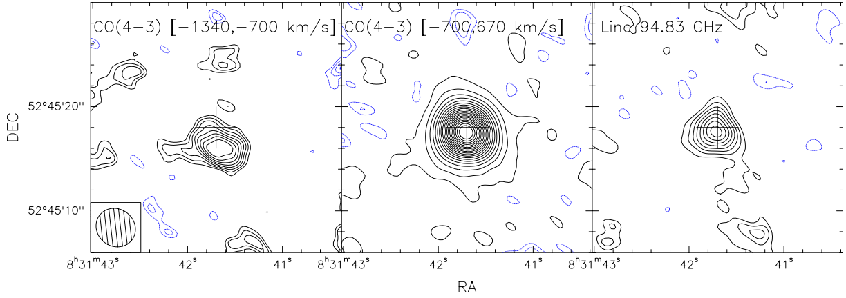
Fig. 4. Left panel: blueshifted CO component is integrated between peak_{blue} - 2\sigma_{blue} = -1340 km s -1 and CO_{sys} - 3\sigma_{sys} = -700 km s -1 (i.e. according to the Gaussian fit in Table 2). Levels start at \pm 2\sigma and increase (decrease) by 0.5\sigma ( \sigma = 39 \mu Jy/beam for an integrated bandwidth of 240 MHz = 767 km s -1 ). Middle panel: the CO systemic line integrated in the range Line - peak \pm 3\sigma is shown. Levels start at \pm 2\sigma and increase (decrease) by 5\sigma ( \sigma = 27.7 \mu Jy/beam for 480 MHz (=1533 km s -1 ) integrated bandwidth). Right panel: the line at 93.85 GHz integrated in the range Line - peak \pm 3\sigma is shown. Levels start at \pm 2\sigma and increase (decrease) by 1\sigma ( \sigma = 34 \mu Jy/beam per 320 MHz = 1022 km s -1 integrated bandwidth). The cross denotes the phase tracking centre and is 4 \times 4 arcsec wide.
