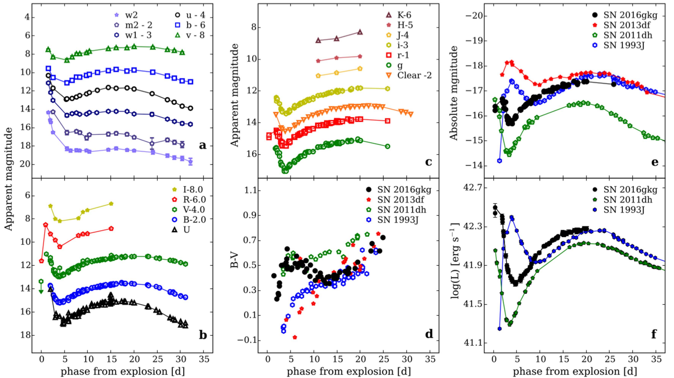
Figure 1. (a) UVOT, (b) UBVRI , and (c) and griJK light curves of SN 2016gkg. (d) B - V color evolution compared with those of SNe 1993J, 2011dh, and 2013df. (e) Absolute r light curves compared with those of SNe 1993J ( R -band), 2011dh ( g -band), and 2013df ( R -band). (f) Pseudo-bolometric light curve compared to those of SNe 2011dh and 1993J. The pseudo-bolometric light curves were computed using Simpson's rule, integrating the photometric data. At early phase only Vr bands are available. For the missing bands, we assumed constant colors and a 10% uncertainty on the computed flux. Errors for SN 2016gkg were computed assuming a fixed distance modulus ( \mu = 32.11 mag). The data used to create this figure are available.
