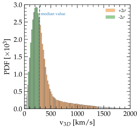
FIG. 8. Distribution of pulsar kick velocities calculated following [86]. The vertical dashed line identifies the median kick velocity.
