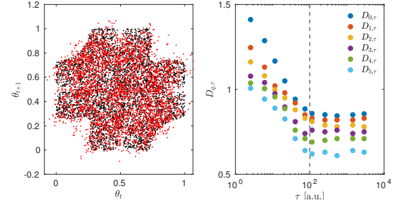
FIG. 5. Left: Phase-space portrait of the standard map as obtained from the raw time series (\theta_t, \theta_{t+1}) (black) and from reconstructions of empirical modes (\theta_t^*, \theta_{t+1}^*) up to k^* = 6 (red). Right: Behavior of the multiscale generalized fractal dimensions D_{q,\tau} vs. the timescale \tau for q \in [0, 5] . The gray dashed line marks the timescale \tau^* at which the multiscale generalized dimensions D_{q,\tau} converge to the fractal dimensions D_q .
