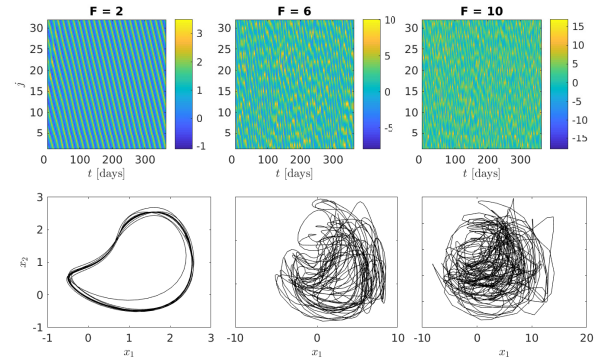
FIG. 8. Top: Contours for a subset of time points corresponding to 1 year of the Lorenz '96 model for three different values of the constant external forcing: (upper left) F = 2 , (upper middle) F = 6 , and (upper right) F = 10 . Bottom: Phase-space portraits of the first two variables (x_1, x_2) for the three different cases: (lower left) F = 2 , (lower middle) F = 6 , and (lower right) F = 10 .
