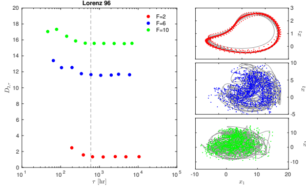
FIG. 9. Left: Behavior of the multiscale correlation dimension D_{2,\tau} vs. the timescale \tau . The gray dashed line marks the timescale \tau^* at which the multiscale correlation dimensions D_{2,\tau} converge to the fractal dimension D_2 . Right: Phase-space portraits of the first two variables of the Lorenz '96 model as obtained from the raw time series (x_1, x_2) (gray) and from reconstructions of empirical modes (x_1^*, x_2^*) up to k^* = 3, 5 , and 6 (red, blue, and green, respectively) for the three different forcing values F = 2, 6 and 10 (from top to bottom), respectively.
