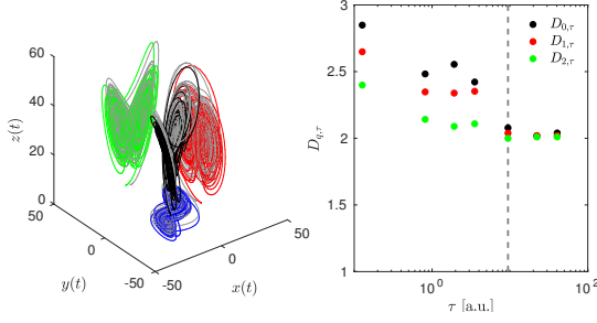
FIG. 4. Left: Phase-space portrait of the Lorenz '63 system based on the raw time series (gray lines) and empirical mode reconstructions (colored lines) by using partial sums of Eq. (12) up to k^* = 5 . Right: Behavior of the multiscale generalized fractal dimensions D_{q,\tau} in dependence on the timescale \tau . The gray dashed line marks the timescale \tau^* at which the multiscale generalized dimensions D_{q,\tau} converge to the expected fractal dimensions D_q .
