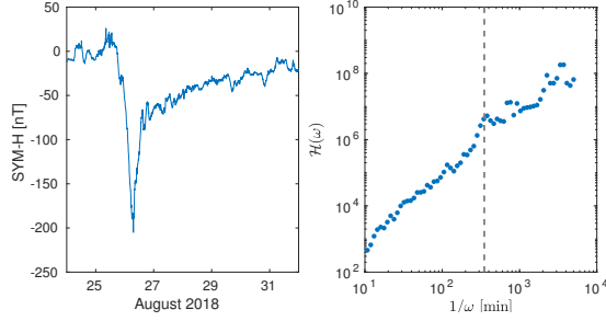
FIG. 13. Left: Time series of the SYM-H index between 24 August and 1 September, 2018. Right: Hilbert marginal spectrum H(\omega) shown as function of 1/\omega .
