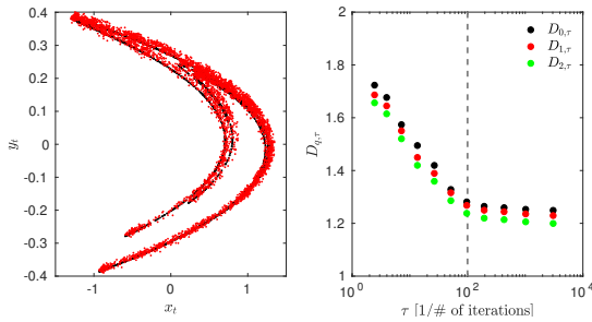
FIG. 1. Left: Phase-space portrait of the H non map based on the raw time series (black) and empirical mode reconstructions (red) using partial sums of Eq. (12) up to k^* = 7 . Right: Behavior of the multiscale generalized fractal dimensions D_{q,\tau} in dependence on the timescale \tau . The gray dashed line marks the timescale \tau^* at which the multiscale generalized dimensions D_{q,\tau} converge to the expected fractal dimensions D_q .
