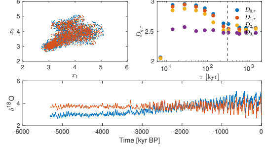
FIG. 12. Top left: Phase-space portrait of the two first embedding components of the LR04 record as obtained by the raw data (blue) and by empirical mode reconstructions (orange) with k^* \in [2, 7] . Top right: Behavior of the multiscale generalized fractal dimensions D_{q,\tau} vs. the timescale \tau for q \in [0, 3] . The gray dashed line marks the timescale \tau^* at which the multiscale generalized dimensions D_{q,\tau} converge to a constant value D_q . Bottom: Time evolution of the \delta^{18}\text{O} stack record during the last 5.3 Myr (blue) and reconstructions of empirical modes (orange) with k^* \in [2, 7] .
