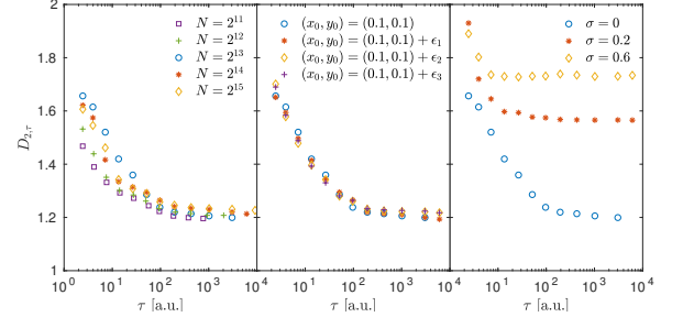
FIG. 2. Behavior of the multiscale generalized fractal dimension D_{2,\tau} for the H non map in dependence on the timescale \tau for different number of iterations N (left panel), different initial conditions (middle panel, N = 2^{13} , \epsilon_i < \epsilon = 0.01 for i = 1, 2, 3 ), and different noise levels \sigma (right panel, N = 2^{13} ).
