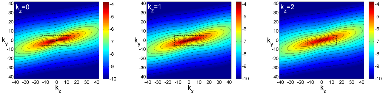
Figure 6. Logarithm of the spectral magnetic energy, \log_{10}\mathcal{E}_M , in (k_x, k_y) -plane at k_z = 0, 1, 2 for the box (4, 4, 1) . The spectra are strongly anisotropic due to the shear, having larger power on the k_x/k_y > 0 side at a given k_y . Dashed rectangles delineate the vital area of turbulence, where the sustaining process is concentrated (see Figures 9-14).
