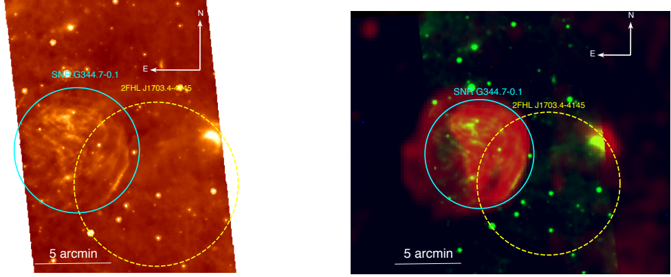
FIG. 5.— Left : SPITZER 24 \mu m image of SNR G344.7-0.1 with 2FHL J1703.4-4145 95% uncertainty region indicated. Note the bright filament on the western edge of the SNR that overlaps well into the 2FHL region. Right : 843 MHz (red) superposed with 24 \mu m (green) and 8 \mu m (blue) SPITZER MIPS and IRAC images, respectively. The bright radio emission is paired with bright IR emission in the center of the SNR. A bright IR filament traces the western edge of the SNR, coincident with the position of 2FHL J1703.4-4145. These two points indicate an interaction between the remnant and its surroundings.
