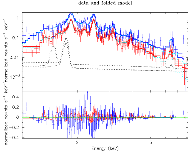
FIG. 3.— Top : XMM-Newton MOS1 and MOS2 (red), and pn (blue) data of the source and background regions (see Figure 2) and the best-fit model (blue and red solid lines) obtained using phabs(vnei + gaussian) . The emission lines observed between 1 keV and 7 keV correspond to metals in the plasma: Mg ( \sim 1.5 keV), Si ( \sim 1.7 keV), S ( \sim 2.4 keV), Ar ( \sim 2.5 keV), Ca ( \sim 4 keV), and Fe ( \sim 6.4 keV) which is consistent with the results reported in Giacani et al. (2011); Yamaguchi et al. (2012) and Fukushima et al. (2020). The dotted dark grey lines correspond to the instrumental background contributions for each data set. The dashed cyan lines correspond to the combination of source and astrophysical background contributions. Bottom : Residual map of the data and best fit model.
