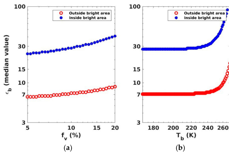
Figure 8. (a) Trend of the median value \varepsilon_b as a function of f_v computed from the posterior pdf p_p(\varepsilon_b^*, f_v^*) inside (blue) and outside (red) the bright area. (b) Trend of the median value \varepsilon_b as a function of T_b computed from the posterior pdf p_p(\varepsilon_b^*, T_b^*) inside (blue) and outside (red) the bright area.
