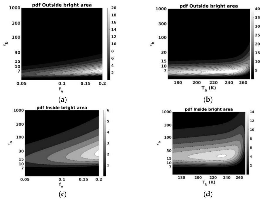
Figure 7. Posterior pdf p_p(\varepsilon_b^*, f_v^*) and p_p(\varepsilon_b^*, T_b^*) outside (a) and (b) and inside (c) and (d) the bright reflector.
