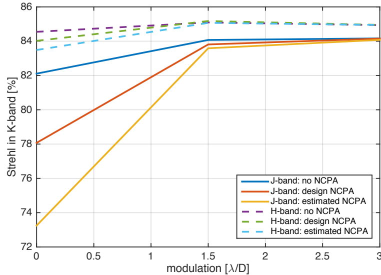
Figure 4. Simulations of the impact of NCPA on the performance (K-band Strehl ratio) of the Keck pyramid at different modulation amplitudes.
