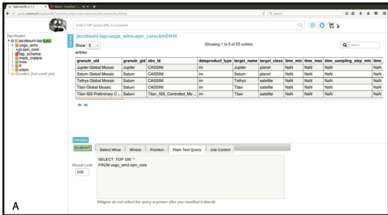
Fig. 9. EPN-TAP table of the USGS planetary maps service, as seen in TapHandle.
