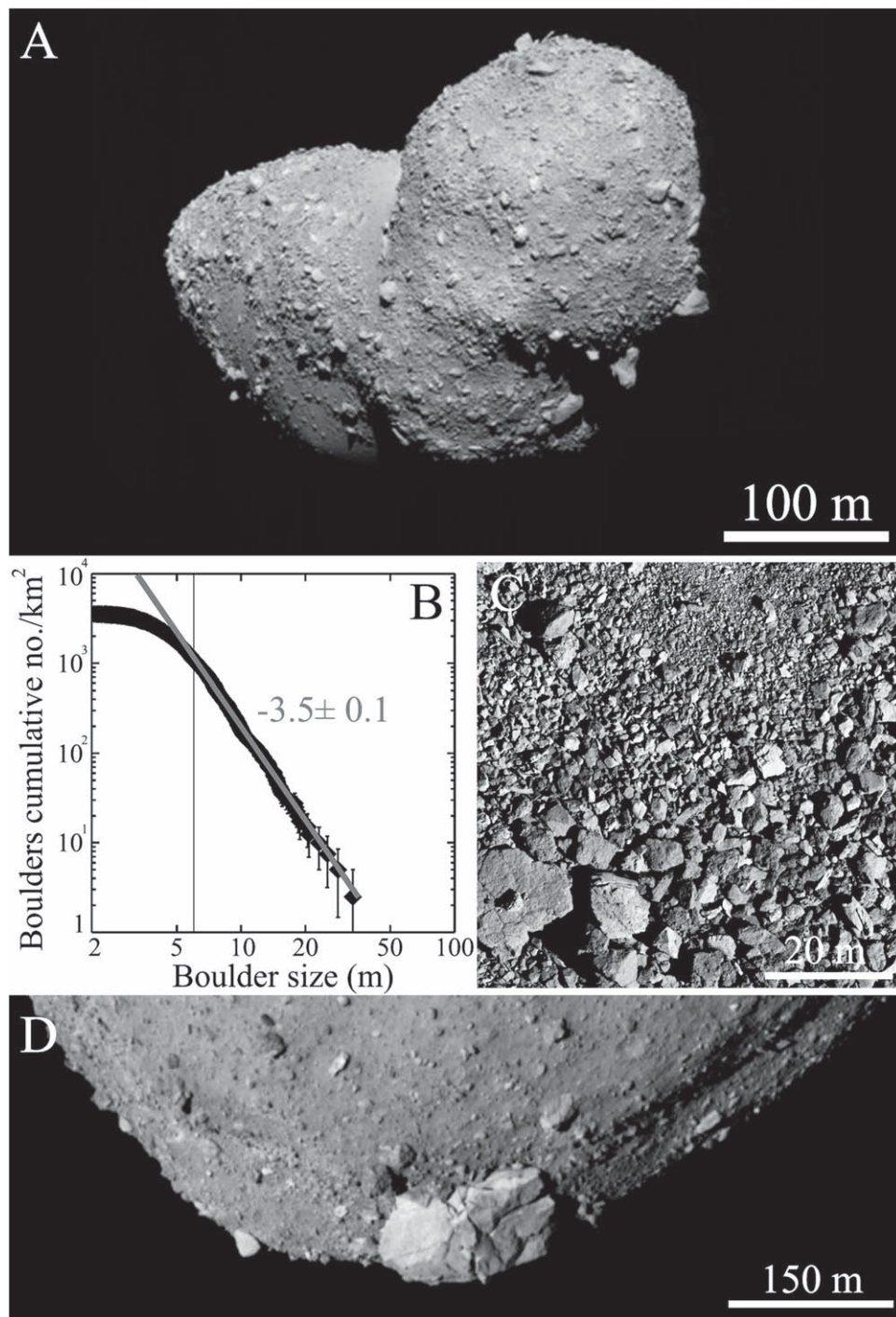
Figure 9. (A) The boulder-rich surface of NEA Itokawa, as observed by Hayabusa. (B) The Itokawa global SFD of boulders as obtained by Mazrouei et al. (2014). (C) Boulders' size grading on Bennu, as observed on a centimeter-scale OCAMS-Polycam (Rizk et al. 2018) image. (D) The southernmost region of asteroid Ryugu. The biggest boulder, called Otohime Saxum, has a size (160 m) that is comparable to the size of Dimorphos.
