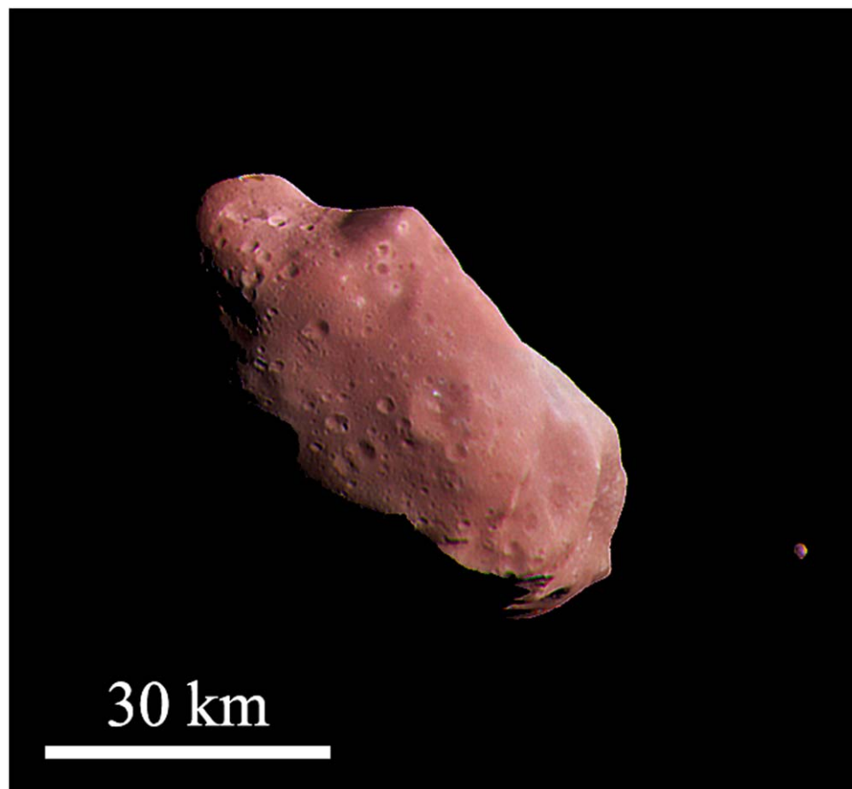
Figure 6. An enhanced-RGB color image obtained on the S-type asteroid Ida and its satellite Dactyl, as obtained by the Galileo mission on 1993 August 28. Thanks to such a data set, a systematic difference between two of Ida’s major color terrains has been identified (Geissler et al. 1996; Veverka et al. 1996), as well as a different spectral trend on Dactyl.
