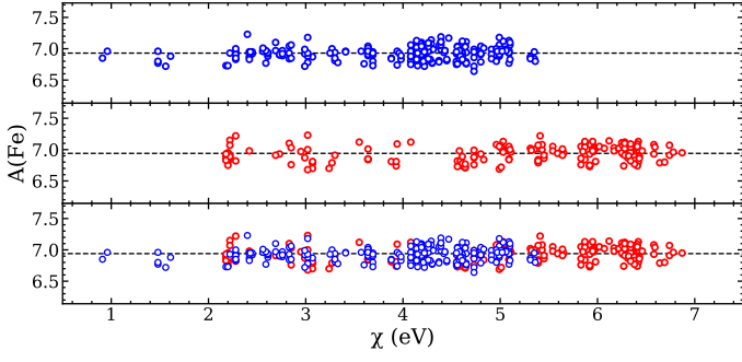
Fig. 5. Iron abundances from neutral lines in the optical UVES spectra (blue circles) and in the NIR GIANO-B spectrum (red circles) as a function of their excitation potential. The dotted line marks the derived best-fit median iron abundance.
