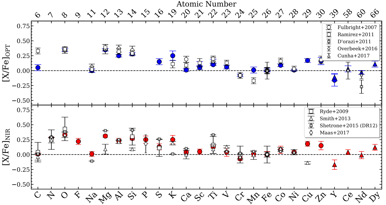
Fig. 10. Derived [X/Fe] chemical abundances for Arcturus from some optical (top panel) and NIR (bottom panel) studies quoted in Table 1 and in Sect. 1. Blue symbols are our abundances from the optical UVES spectra, and red symbols our abundances from the NIR GIANO-B spectrum. Blue and red dots refer to neutral species, and blue and red triangles to ionised species.
