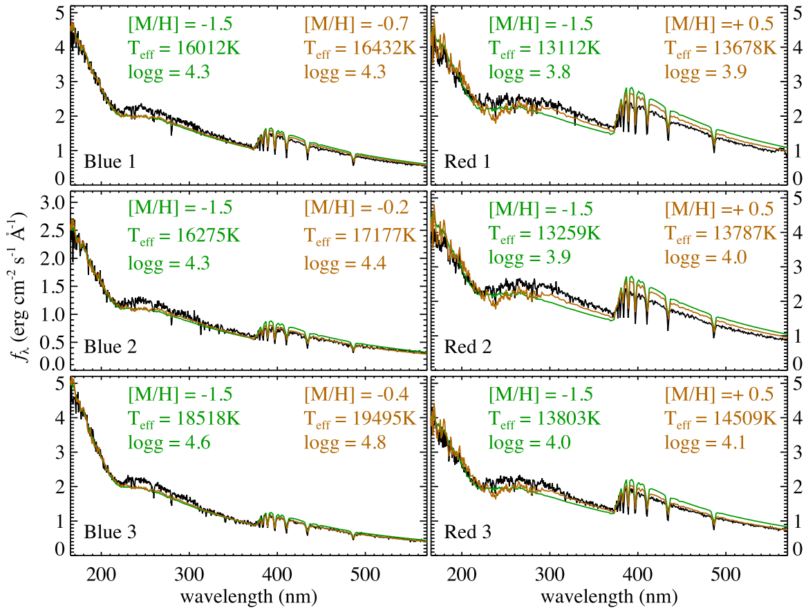
Figure 6. Spectra of our six stars (black curves) compared to the best-fit synthetic spectra (colored curves) from the Castelli & Kurucz (2003) grid. In all of the fits, the effective temperature is allowed to float, and the surface gravity is fixed at the value corresponding to that temperature along the zero-age horizontal branch. The extinction is fixed at E(B - V) = 0.13 mag (Bellini et al. 2017b; Milone et al. 2017b). Neither the fits with the metallicity at the mean cluster value ( [M/H] = -1.5 ; Harris 1996; green curves) nor the fits with the metallicity allowed to float (labeled; brown curves) are able to match the general shape of the pseudo-continuum and the size of the Balmer jump, although the models with floating metallicity perform somewhat better. Even with the poor fits shown here, the synthetic spectra imply that the red stars are \sim 2000 – 4000 K cooler than the blue stars, and that the red stars have a greater enhancement of atmospheric metallicity due to radiative levitation. Note that the upper metallicity limit in the Castelli & Kurucz (2003) grid is +0.5 dex.
