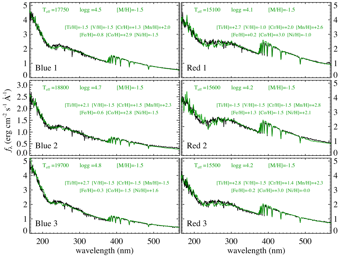
Figure 7. Spectra of our six stars (black curves) compared to the best-fit synthetic spectra (green curves) from ATLAS12 and SYNTHE. In these models, most elements are held at the mean cluster abundance ( [M/H] = -1.5 ; Harris 1996), but seven elements (labels) near the Fe peak are allowed to vary up to an enhancement of 4.5 dex over the cluster value, because they can be significantly affected by radiative levitation (Michaud et al. 2011). The best-fit values in each fit (labels) are shown in Figure 8 to ease comparisons. The changes induced on each spectrum by the enhanced atmospheric metallicities are much larger in the red stars than in the blue stars (Figure 9).
