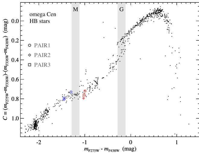
Figure 1. WFC3 photometry (black points) of HB stars in \omega Cen (Bellini et al. 2017a), shown as a color–color diagram that makes it easy to discern the G-jump and M-jump (labeled; as in Brown et al. 2016). The ordinate is a color index ( C ) that is useful for discerning changes in the stellar atmosphere (in the hot stars here but also the cooler stars studied in the multiple populations phenomenon). For our investigation, we obtained STIS near-UV (G230L) and blue (G430L) spectroscopy of six stars (colored symbols matching those in Figure 2) that straddle the M-jump, with wavelength coverage that includes the three photometric bands employed in this color–color diagram (F275W, F336W, and F438W). If the photometry here is aligned to a theoretical zero-age HB locus (see Brown et al. 2016), the gray band representing the M-jump spans \sim 15,000 – 18,000 K in effective temperature.
