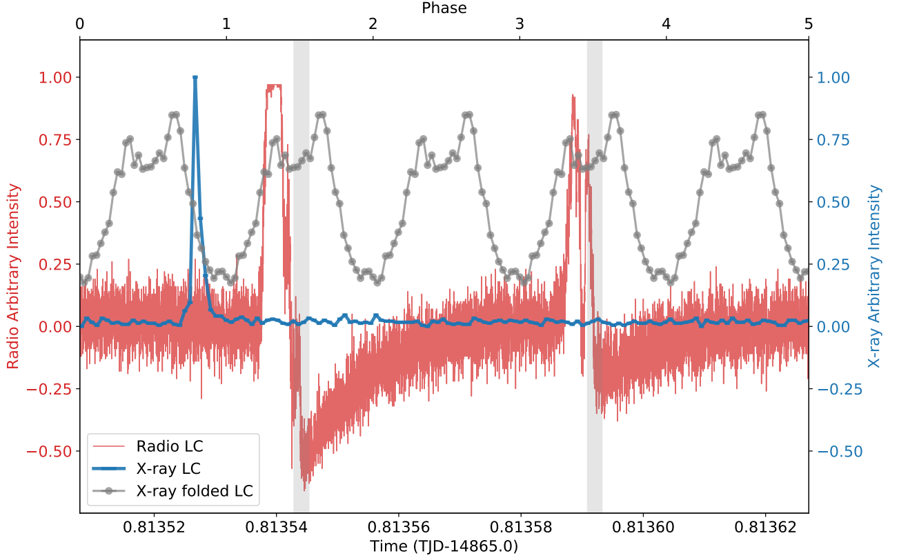
Figure 3. X-ray and radio simultaneous observations of 1E 1547.0–5408 performed on 2009 February 3, around the time of the brightest X-ray burst (burst “2” in Fig. 1) and the two radio pulses (pulse A and B). The blue line is the burst lightcurve, while the grey line is the X-ray folded light curve using the XMM-Newton dataset. The Parkes simultaneous radio light curve is shown in red. The grey shaded areas are the phase intervals of the expected peak of the radio pulse profiles extrapolated from the 2009 January 25 Parkes observation (see also Figure 2). Note that the flat top of the first radio peak (pulse A), and the drop of the intensity of the radio signal below the average noise level following both pulses, are artifacts caused by the saturation of the backend.
