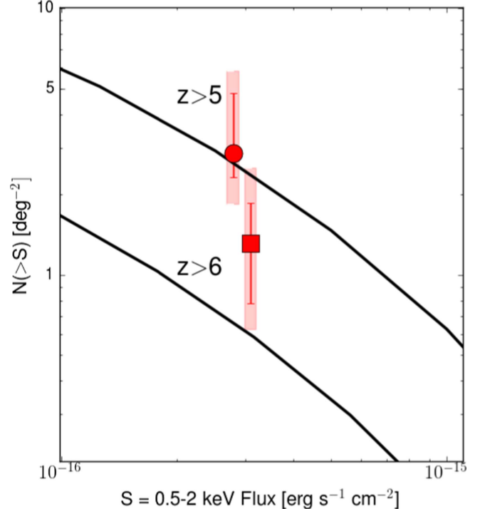
Figure 8. LogN-LogS relation in the 0.5–2 keV band for Chandra COSMOS-Legacy (red circles), for z > 5 (upper part) and z > 6 (lower part). Models from Gilli et al. (2007, black solid line) are also shown for comparison. The pale red area is obtained by computing the number counts adding and subtracting to the flux value its 1\sigma error. In the computation of the upper boundary, the weighted contribution of sources with no optical counterpart is also taken into account.
