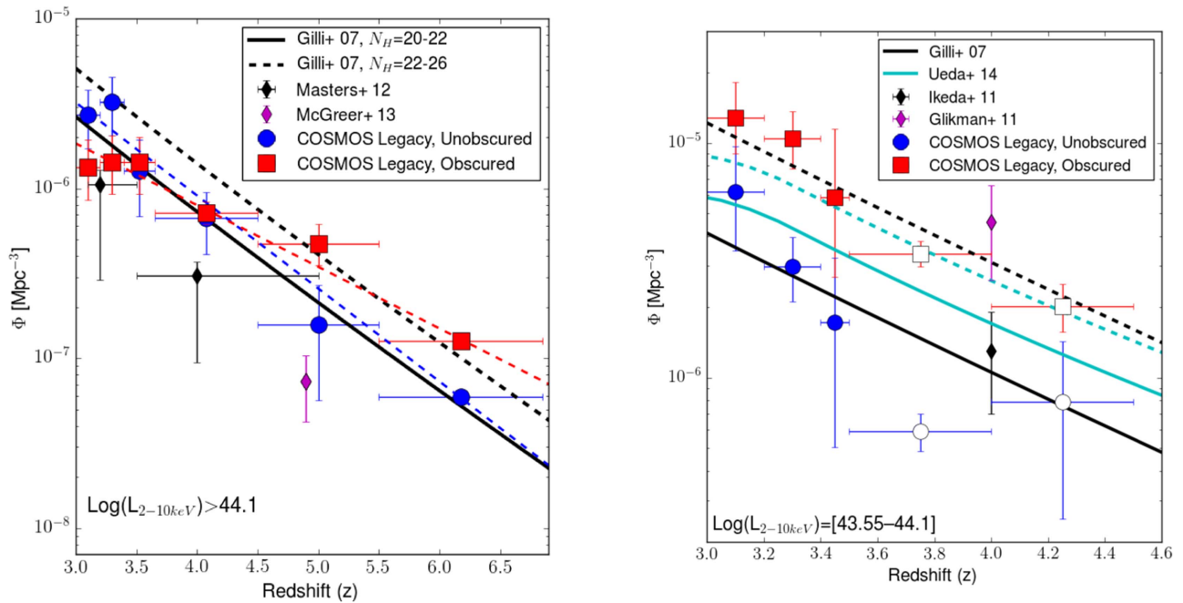
Figure 11. Space density for sources with L_X > 10^{44.1} (left) and 10^{43.55} \leq L_X < 10^{44.1} (right) in the 2–10 keV band. The sample of type 1 AGNs is plotted with blue dots, while the sample of type 2 AGNs is plotted with red squares. The blue and red dashed lines in the left panel are the best fit to the Type 1 and Type 2 samples, respectively, assuming the equation \text{Log}(\Phi) = a + b \times z . The model of X-ray population synthesis from Gilli et al. (2007) is also shown, one with N_H = [20-22] (black solid line) and the other with N_H = [22-26] (black dashed line); the model from Ueda et al. (2014) is shown in cyan for N_H = [20-22] (solid line) and N_H = [22-24] (dashed line). Optical space densities from Masters et al. (2012, black diamonds, left; Type 1 AGNs only), McGreer et al. (2013, magenta diamonds, left; Type 1 AGNs only), Ikeda et al. (2011, black diamonds, right), and Glikman et al. (2011, magenta diamonds, right) are also shown for comparison. The open markers in the right panel are the results obtained in those redshift bins where our survey is not complete, and therefore should be treated as lower limits.
