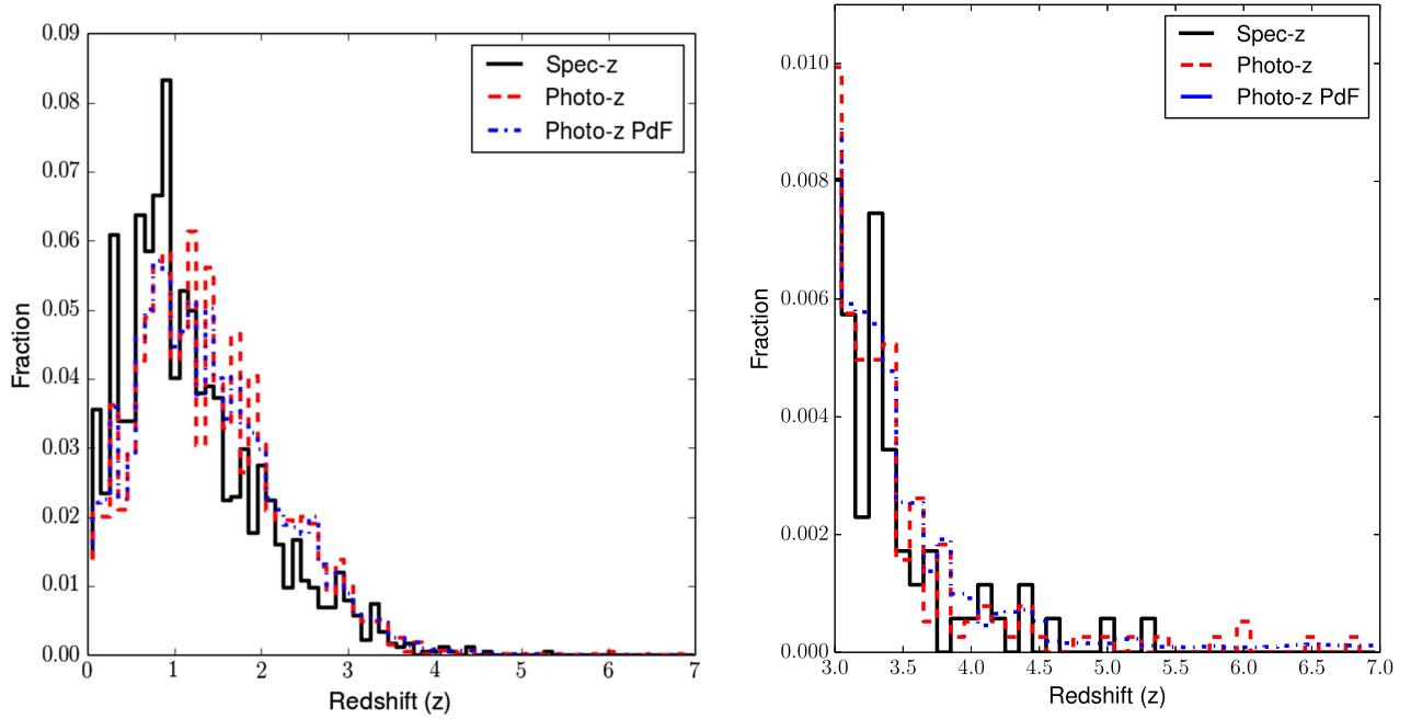
Figure 1. Normalized distributions of redshift for sources with a spectroscopic redshift (black solid line), for photometric redshifts PDF peak value z_{\text{peak}} (red dashed line), and for the PDF of all sources with a photometric redshift (blue dashed-dotted line) for (left) all of the sources in the Chandra COSMOS-Legacy and (right) for the high-redshift sample at z \geq 3 . The agreement between the photometric redshift z_{\text{peak}} distribution and the distribution of the PDFs is good at all redshifts, which means that the majority of source have narrow and highly peaked PDF.
