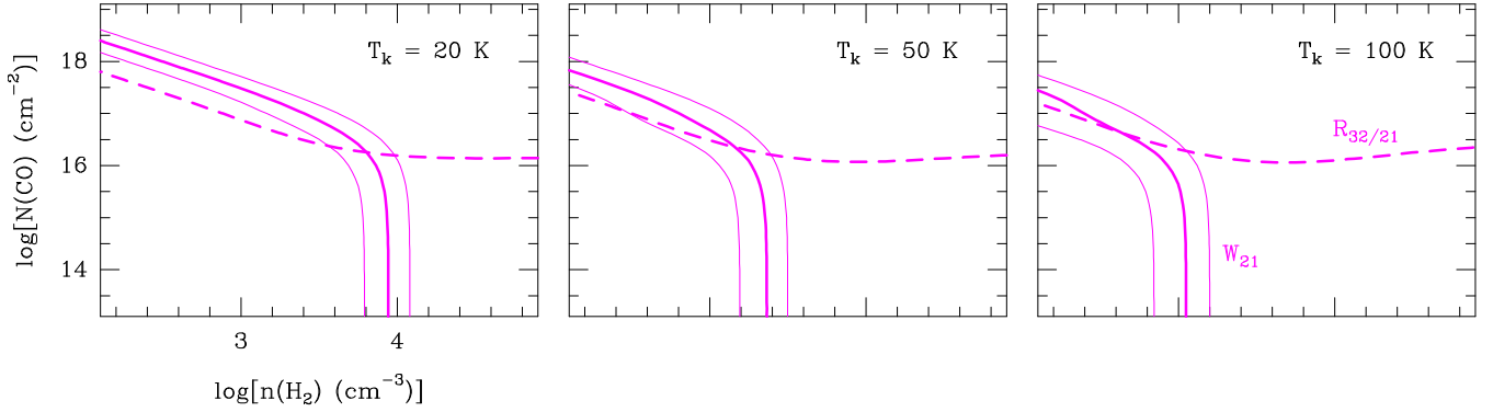
Figure 8. Results of RADEX fitting for T_k = 20 K, T_k = 50 K and T_k = 100 K. Dashed contours represent the measured CO (3 \rightarrow 2)/(2 \rightarrow 1) ratio; solid contours represent the CO J = 2 \rightarrow 1 integrated intensity, with its uncertainties. The intersection of the two sets of contours indicate the range of possible values for n(\text{H}_2) and N(\text{CO}) .
