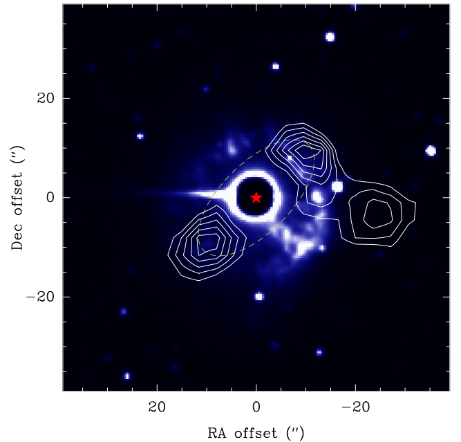
Figure 10. Relative orientation of the optical jet and the molecular ring. ESO/SC1 coronagraphic continuum image of AG Car and its nebula in color scale (Vamvatira-Nakou et al. 2015). ACA+TP CO J = 2 \rightarrow 1 intensity map superimposed as contours. Contours start at 50% of the peak intensity, showing only the ring blobs, for the sake of clarity. The dashed ellipse is displayed to highlight the extent of the structure. The red marker indicates the position of the star. The bright spike to the east is an imaging artefact.
