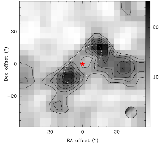
Figure 3. ACA+TP velocity-integrated intensity map of CO J = 2 \rightarrow 1 towards AG Car, in the velocity range (+29, +36) km s ^{-1} . Contours start at 8 K km s ^{-1} in steps of 2.5 K km s ^{-1} . The red marker indicates the position of the star, and the hatched circle in the bottom right corner represents the ACA synthesized beam size. The dashed ellipse represents the ellipse used for the fitting.
